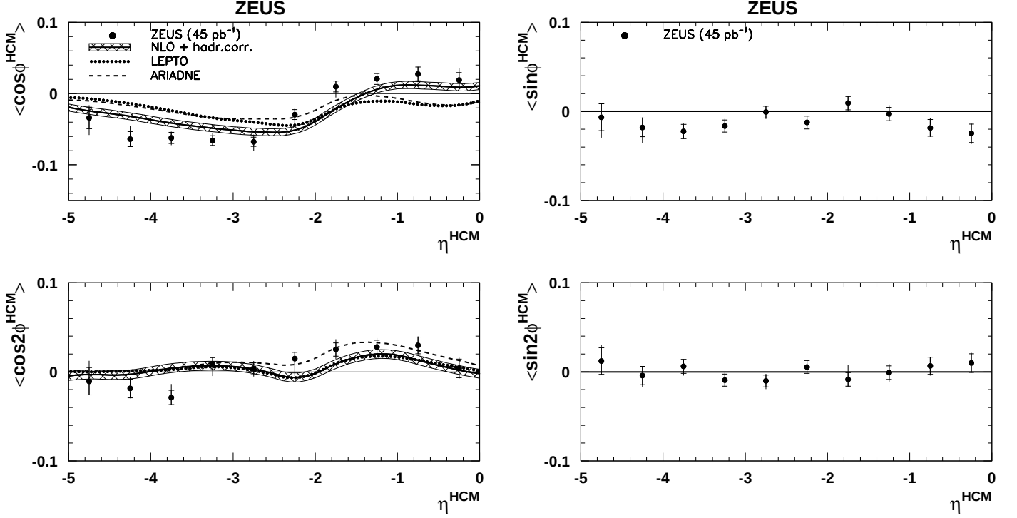
Figure 3: The values of \langle \cos \phi^{HCM} \rangle , \langle \cos 2\phi^{HCM} \rangle , \langle \sin \phi^{HCM} \rangle and \langle \sin 2\phi^{HCM} \rangle , calculated using the energy-flow method as in Eq. (2), as a function of hadron pseudorapidity, \eta^{HCM} . They were obtained in the HCM frame for the kinematic region 100 < Q^2 < 8000 \text{ GeV}^2 , 0.01 < x < 0.1 and 0.2 < y < 0.8 for hadrons with p_T > 0.15 \text{ GeV} and \theta > 8^\circ . The inner error bars are statistical uncertainties, the outer are statistical and systematic uncertainties added in quadrature. The NLO QCD predictions of DISENT (solid line), with its associated uncertainty (shaded band), corrected for hadronisation and hadron losses (see text), the predictions of LEPTO 6.5.1 (dotted line), and the predictions of ARIADNE 4.12 (dashed line) are shown.
