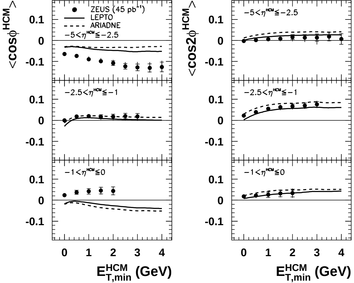
Figure 4: The values of \langle \cos \phi^{HCM} \rangle and \langle \cos 2\phi^{HCM} \rangle , calculated using the energy-flow method as in Eq. (2), as a function of hadron minimum transverse energy, E_{T,min}^{HCM} . They were obtained in the HCM frame for the pseudorapidity intervals -5 < \eta^{HCM} \le -2.5 , -2.5 < \eta^{HCM} \le -1 and -1 < \eta^{HCM} \le 0 in the kinematic region 100 < Q^2 < 8000 \text{ GeV}^2 , 0.01 < x < 0.1 and 0.2 < y < 0.8 for hadrons with p_T > 0.15 \text{ GeV} and \theta > 8^\circ . The inner error bars are statistical uncertainties, the outer are statistical and systematic uncertainties added in quadrature. The predictions of LEPTO 6.5.1 (solid line) and of ARIADNE 4.12 (dashed line) are shown.
