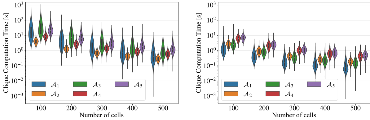
(a) one-to-many algorithm ( D_{pRegLC} ) (b) many-to-many algorithm ( lcD_{pRegLC} )
