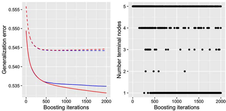
Figure 8. In-sample (solid blue line for ABT, solid red line for GBT) and out-of-sample (dotted blue line for ABT, dotted red line for GBT) estimates of the generalization error for J = 5 and \beta = 99\% (left panel) and number of terminal nodes of the constituent trees for ABT (right panel).
