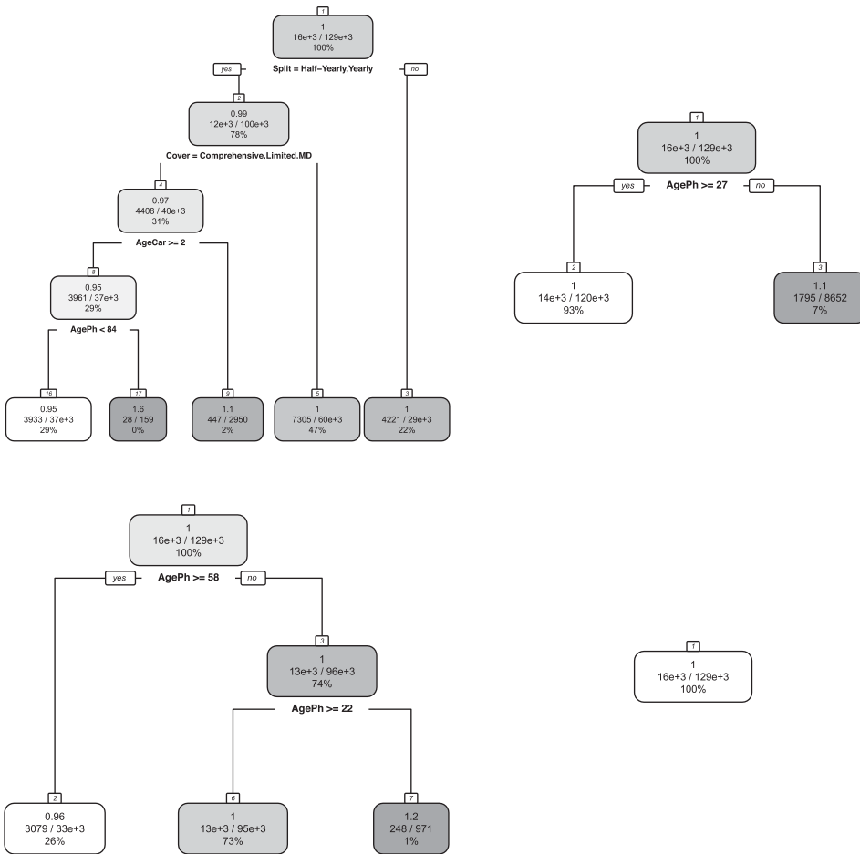
Figure 6. Trees at iteration 306 (top-left), 307 (top-right), 308 (bottom-left) and 309 (bottom-right).
