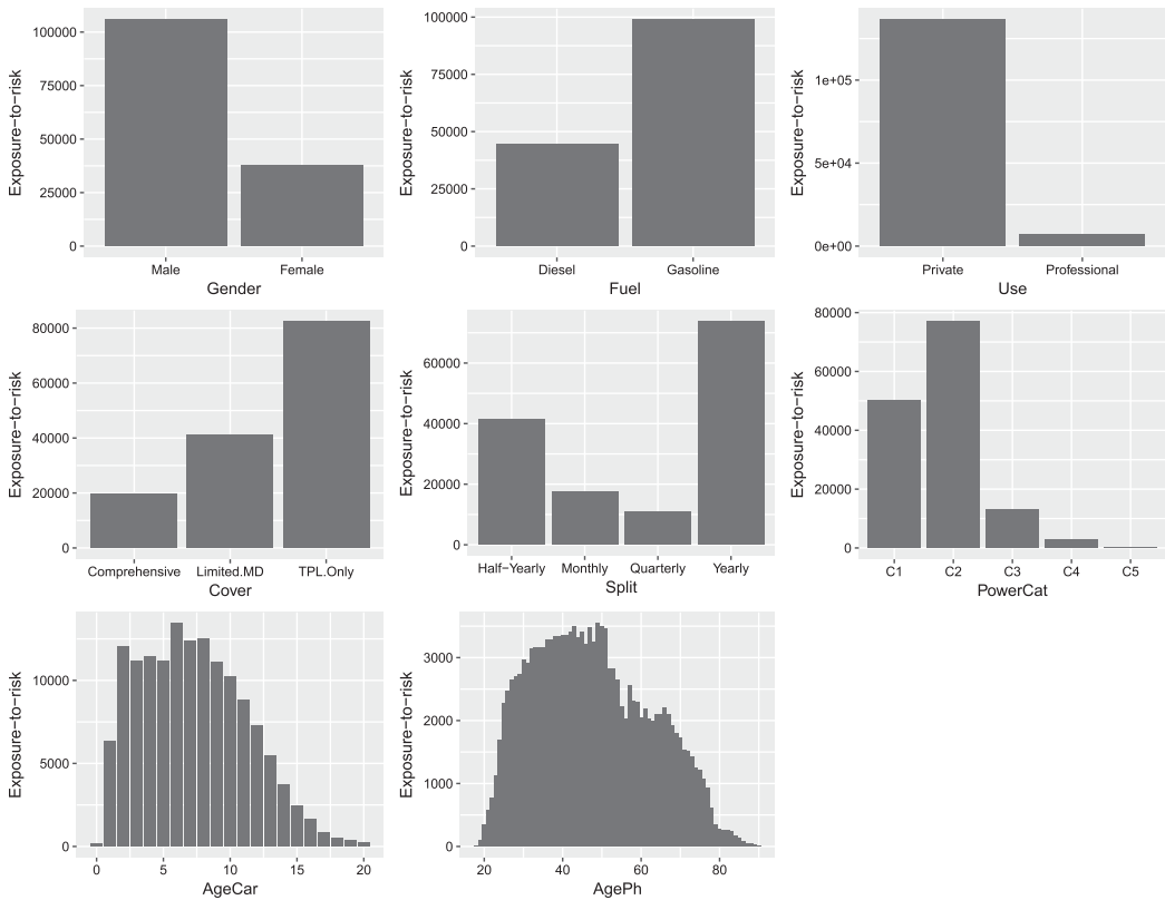
Figure 2. Levels/values of the features and corresponding exposures-to-risk.
