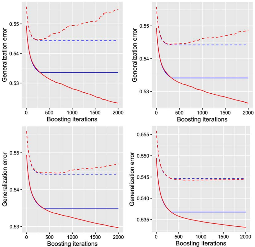
Figure 3. In-sample (solid blue line for ABT, solid red line for GBT) and out-of-sample (dotted blue line for ABT, dotted red line for GBT) estimates of the generalization error for J = 20 (upper left panel), J = 15 (upper right panel), J = 10 (bottom left panel), and J = 5 (bottom right panel).
