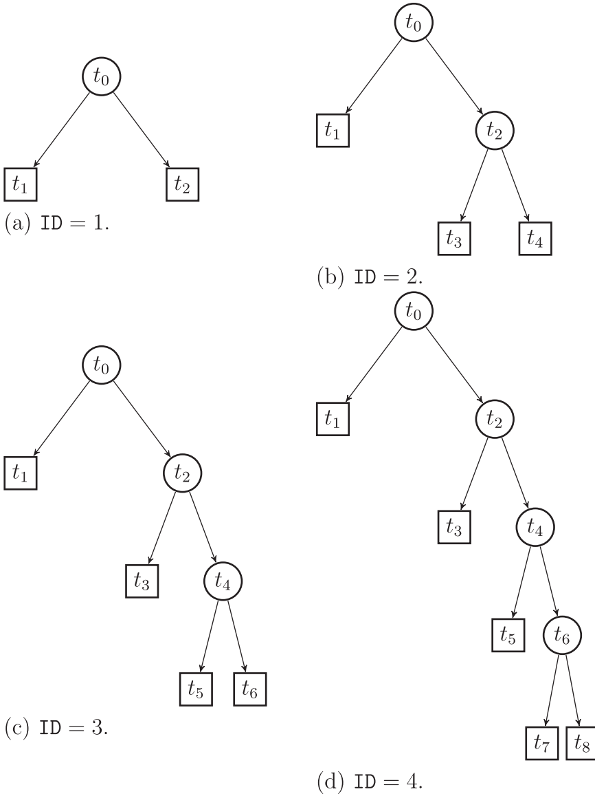
Figure 1. Example of binary regression trees with ID = 1, 2, 3, 4. Circles indicate non-terminal nodes and square boxes represent terminal nodes. (a) ID = 1, (b) ID = 2, (c) ID = 3 and (d) ID = 4.
