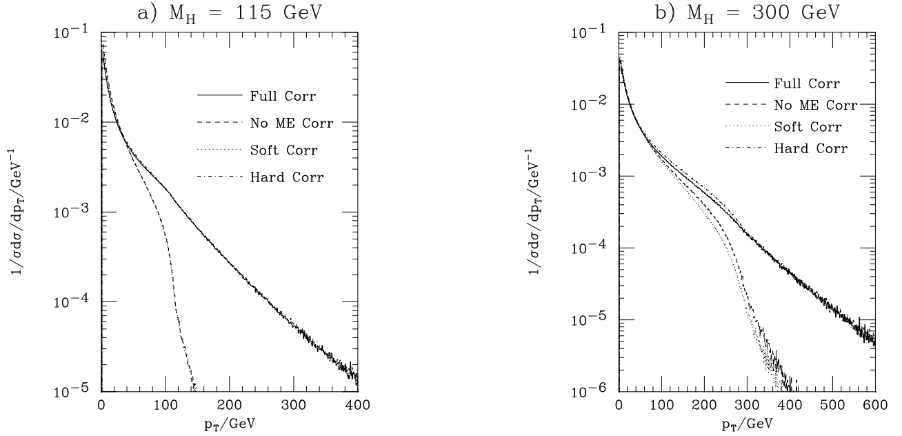
Figure 1: The transverse momentum of the Higgs boson at the LHC for a Higgs boson with mass a) 115 GeV and b) 300 GeV. The results of the full correction (solid), no correction (dashed), only the soft matrix element correction to radiation generated by the parton shower (dotted), and the hard correction filling the ‘dead’ region not filled by the parton shower (dot-dashed) are shown.
