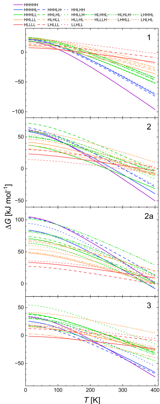
Fig. 5 Calculated temperature dependence of \Delta G of the spin transition from the LLLLL spin isomers to all spin isomers of heptanuclear model of 1, 2, 2a and 3 obtained with B3LYP/D3 functional.
