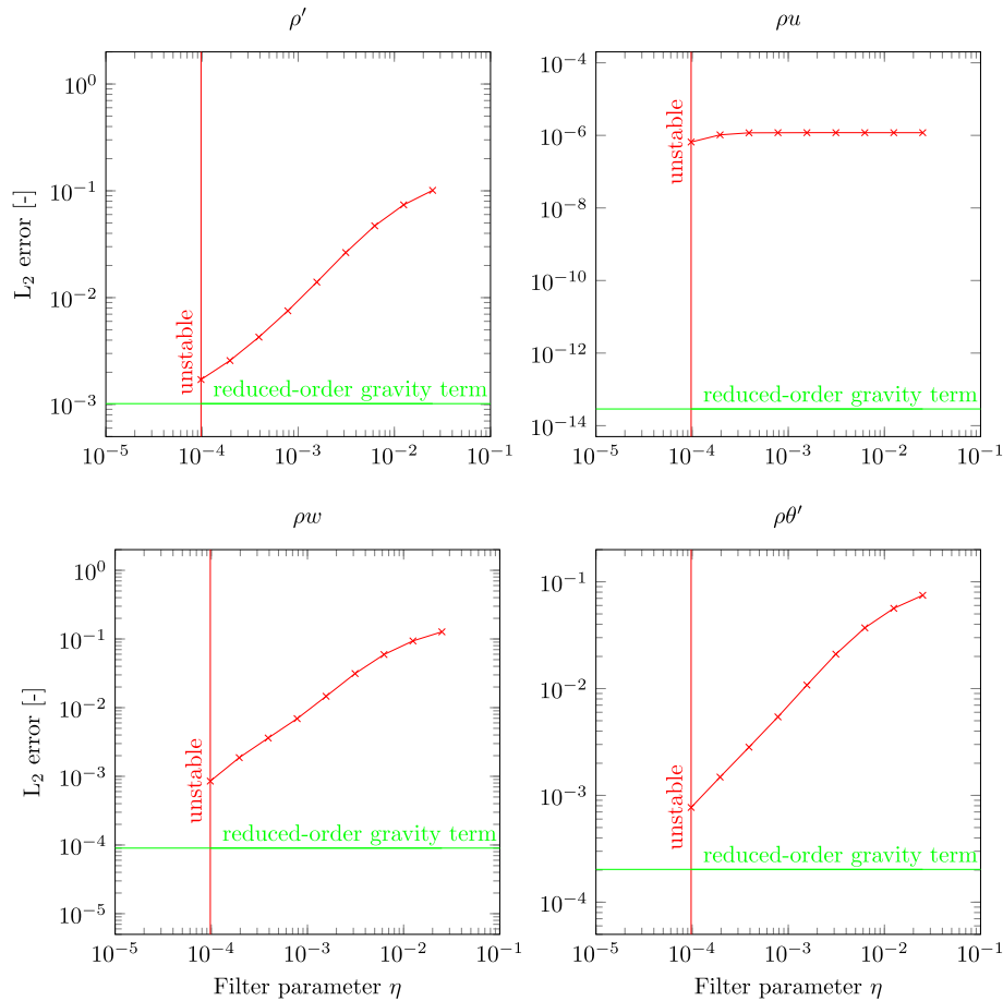
Figure 8. Gravity waves on an anisotropic mesh: L_2 error after 30 min for the prognostic variables, using the reduced-order gravity term (green), and the regular gravity term stabilized using a Boyd–Vandeven filter with several values of the parameter \eta (red). The vertical red lines corresponds to the minimum value of \eta under which the simulations are not stable (model crash).
