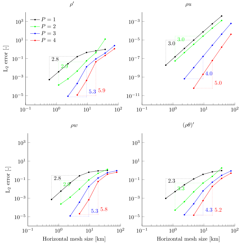
Figure 4. Gravity waves: spatial convergence of the L_2 error after 30 min for the prognostic variables, using spatial polynomial orders P from one to four.
