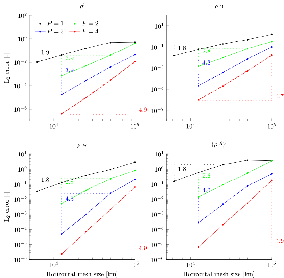
Figure 11. Three-dimensional box with analytical solution: spatial convergence of the L_2 error after T = 100 s for the prognostic variables, using spatial polynomial orders P from one to four.
