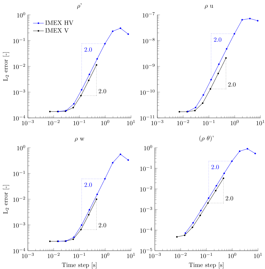
Figure 10. Gravity waves: temporal convergence of the L_2 error after 30 min for the prognostic variables, using respectively the second order IMEX HV and IMEX V time discretizations. Fifth order polynomials are used for the spatial discretization.
