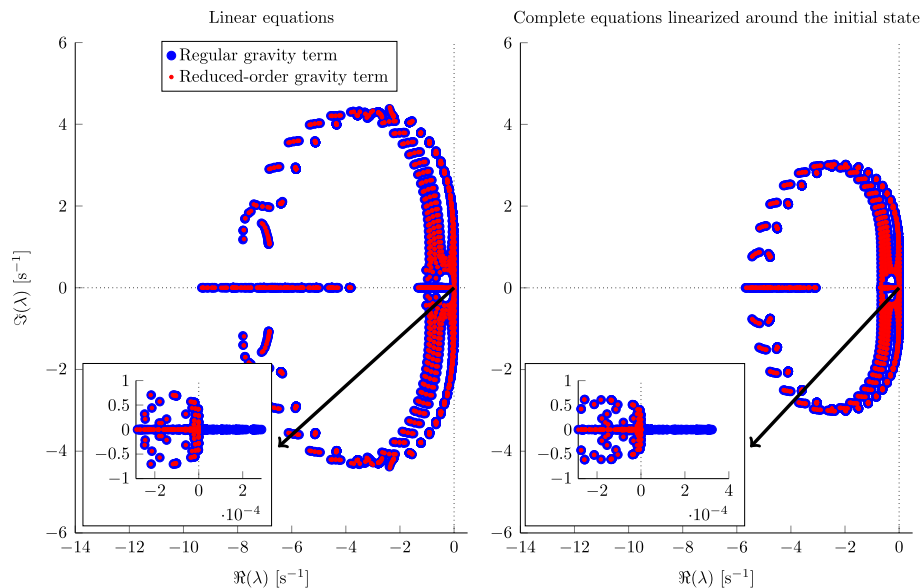
Figure 7. Original gravity waves test case from [55]: eigenvalues \lambda of the discrete spatial operator for simulations with the regular gravity term (blue) and the reduced-order gravity term (red). This spatial operator corresponds to the linear equations (17) for the left plot and the complete equations (4) linearized around the initial condition for the plot on the right. The inner plots show a zoom for real parts of the eigenvalues lying around zero. The solution was computed using third-order polynomials on 8 \times 8 elements.
