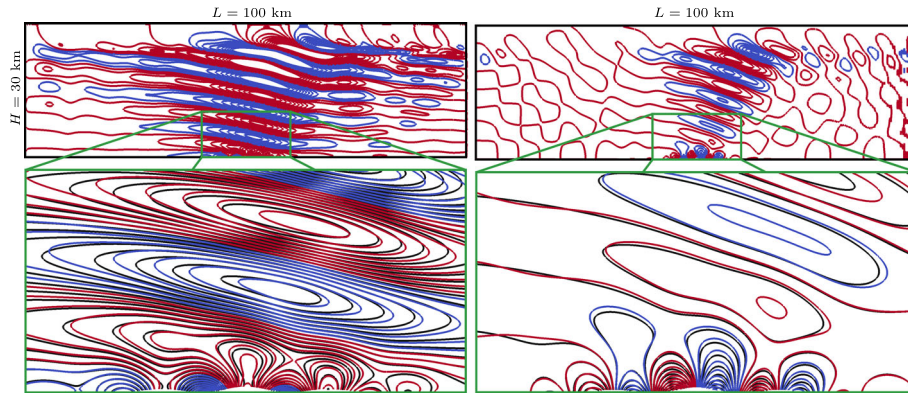
Figure 15. Schär mountain: numerical solution (blue negative, red positive) and analytical solution (black) after 5 h. Contour lines for the horizontal velocity perturbation u - 10 \text{ ms}^{-1} (left) and vertical velocity w (right) every 0.2 \text{ ms}^{-1} from -0.2 to 2 \text{ ms}^{-1} . Solution computed using third-order polynomials on 133 \times 47 elements, corresponding to approximate effective horizontal and vertical resolutions of respectively 250 and 210 m.
