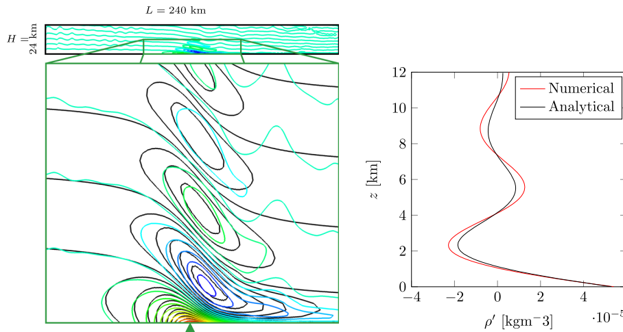
Figure 16. Flow past a three-dimensional linear hydrostatic mountain: density deviation \rho' after 5 h. Left: contour lines every 5 \cdot 10^{-6} \text{ kgm}^{-3} from -2.5 to 5.5 \cdot 10^{-5} \text{ kgm}^{-3} for the model simulation (color) and analytical solution (black). Right: vertical profile at x = y = 0 . Solution computed using third-order polynomials on 53 \times 53 \times 26 elements, corresponding to approximate effective horizontal and vertical resolutions of respectively 1 500 and 310 m. The green triangle indicates the location of the mountain.
