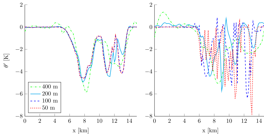
Figure 13. Density current: potential temperature perturbation \theta' after 900 s at different resolutions using a background diffusion (left) or the Boyd–Vandeven filter (right). The figure displays profiles at the height z = 1\,200 m.
