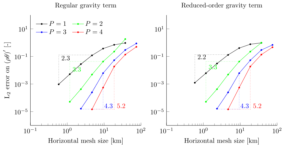
Figure 9. Gravity waves without and with vertical order reduction of the gravity term: spatial convergence of the L_2 error on (\rho\theta)' after 30 min, using spatial polynomial orders P from one to four.
