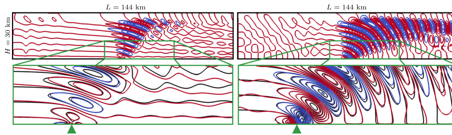
Figure 14. Flow past a nonhydrostatic mountain: numerical solution (blue negative, red positive) and analytical solution (black) after 5 h. Contour lines for the horizontal velocity perturbation ( u - 10 \text{ ms}^{-1} ) every 0.0025 \text{ ms}^{-1} from -0.025 \text{ ms}^{-1} to 0.025 \text{ ms}^{-1} (left). Contour lines for the vertical velocity ( w ) every 0.0005 \text{ ms}^{-1} from -0.005 \text{ ms}^{-1} to 0.005 \text{ ms}^{-1} (right). Solution computed using third-order polynomials on 133 \times 33 elements, corresponding to approximate effective horizontal and vertical resolutions of respectively 360 and 300 m. The green triangle indicates the location of the mountain.
