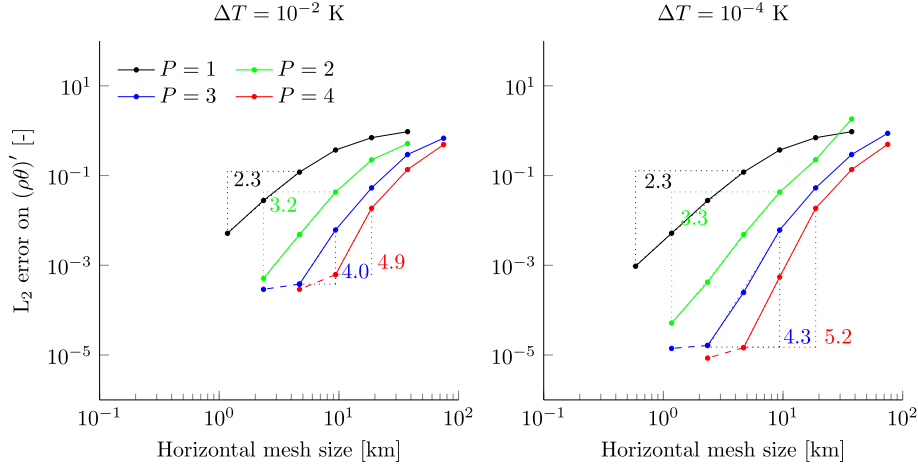
Figure A1. Gravity waves with \Delta T = 10^{-2} K and \Delta T = 10^{-4} K: spatial convergence of the L_2 error on (\rho\theta)' after 30 m, using spatial polynomial orders P from one to four.
