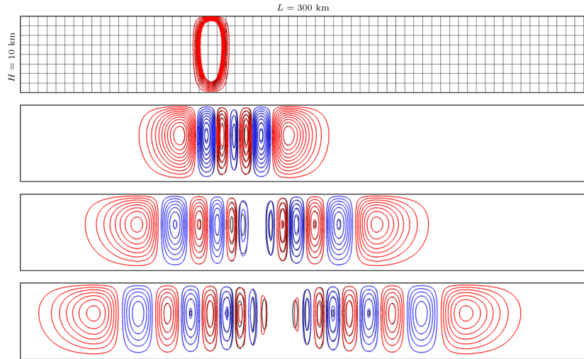
Figure 2. Gravity waves: potential temperature deviation \theta' after 0, 10, 20 and 30 min (from top to bottom). Contour lines every 0.0005 K from -0.005 to 0.005 K, without the zero contour, for the model simulation (blue negative, red positive) and analytical solution (black). The solution was computed using third-order polynomials on 64 \times 8 elements. For visualization purposes, the domain is vertically stretched by a factor of 4. As the model solution is close to the analytical solution, the difference between them is only visible for the largest times (lower panels).
