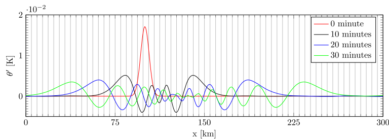
Figure 3. Gravity waves: potential temperature deviation \theta' after 0, 10, 20 and 30 min. The figure displays profiles at mid-height z = 5\,000 m.
