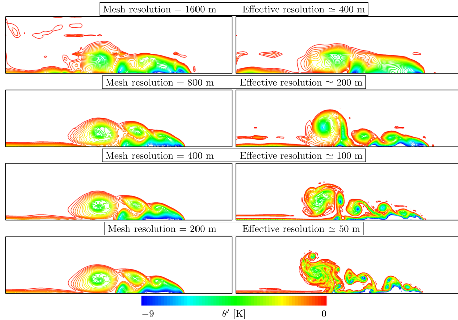
Figure 12. Density current: potential temperature perturbation \theta' after 900 s at different resolutions using a background diffusion (left) or the Boyd–Vandeven filter (right). Contour lines every 0.25 K from -9 to -0.25 K. Only a part of the domain is displayed, corresponding to the interval [0, 19200] \times [0, 4800] m.
