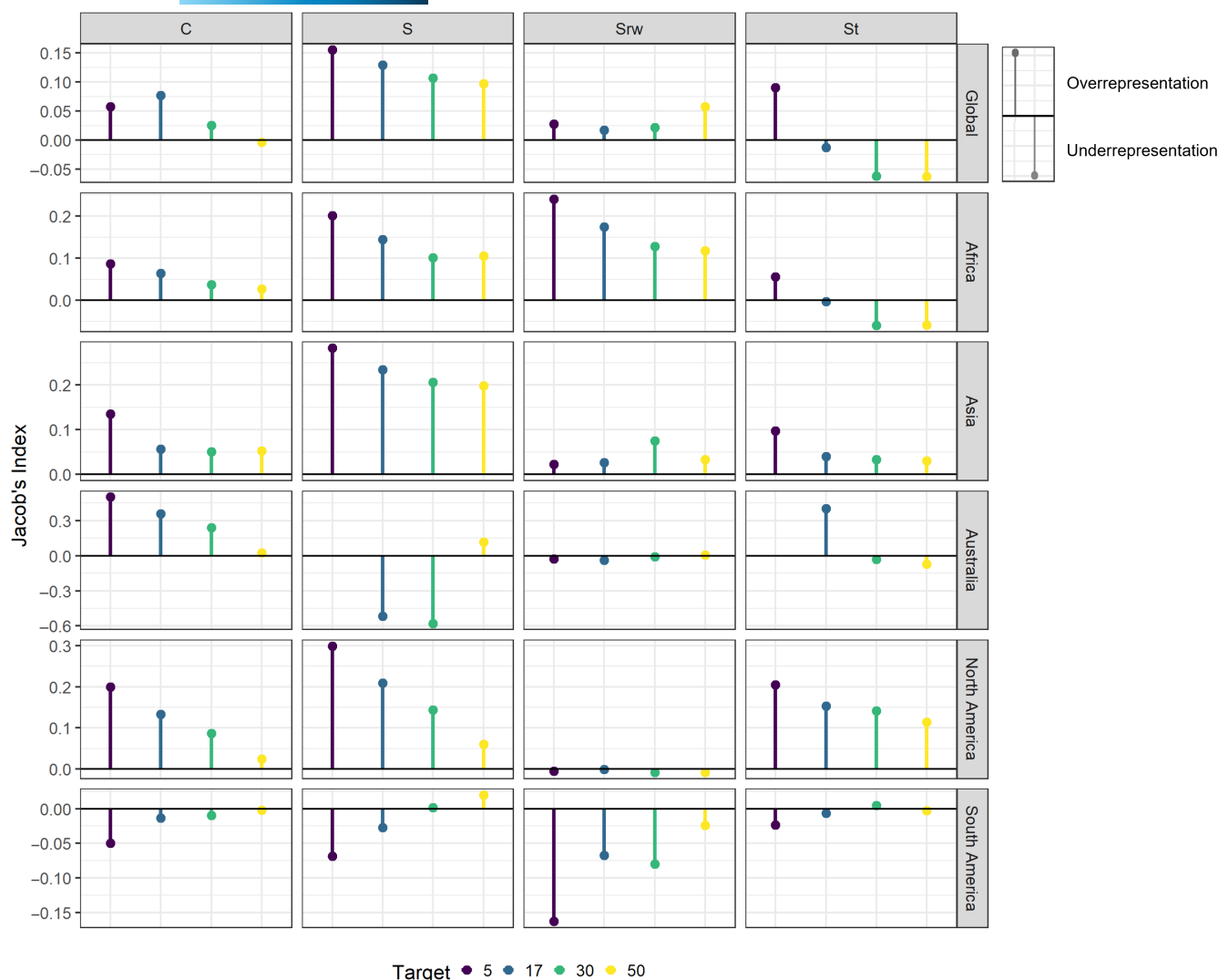
FIGURE 5 Selection index of target areas (5%, 17%, 30% and 50%) for our regional conservation assets of grid cells under deforestation frontiers for tropical dry woodlands globally and within continents. (Regional conservation assets: Carbon, S—total woodland species richness, Sw—the range-weighted rarity of woodland species and St—threatened woodland species richness. 'Overrepresentation' means that the areas within a given target area of the asset for a certain indicator within a certain region have a higher share under deforestation frontiers than the neutral expectation (i.e. the 41% overall share of frontier areas in global tropical dry woodlands).
