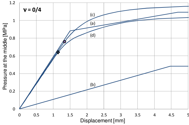
Figure 5. Pressure displacement relationships for \nu = 0/4 . Solutions for: (a) cosinusoidal pressure profile; (b) sinusoidal pressure profiles; (c) F.E. solution without section reduction due to the rivet hole; (d) F.E. solution with section reduction due to rivet hole.
