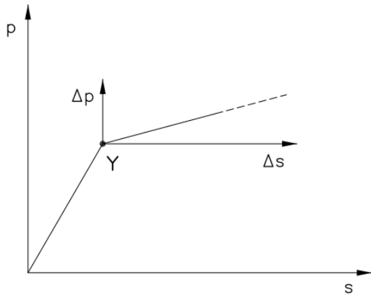
Figure 4. Superposition of the plastic phase to the elastic one.
