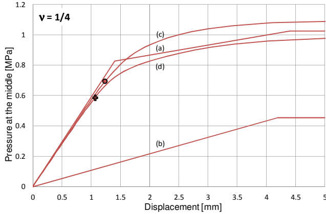
Figure 6. Pressure displacement relationships for \nu = 1/4 . Solutions for: (a) cosinusoidal pressure profile; (b) sinusoidal pressure profiles; (c) F.E. solution without section reduction due to the rivet hole; (d) F.E. solution with section reduction due to rivet hole.
