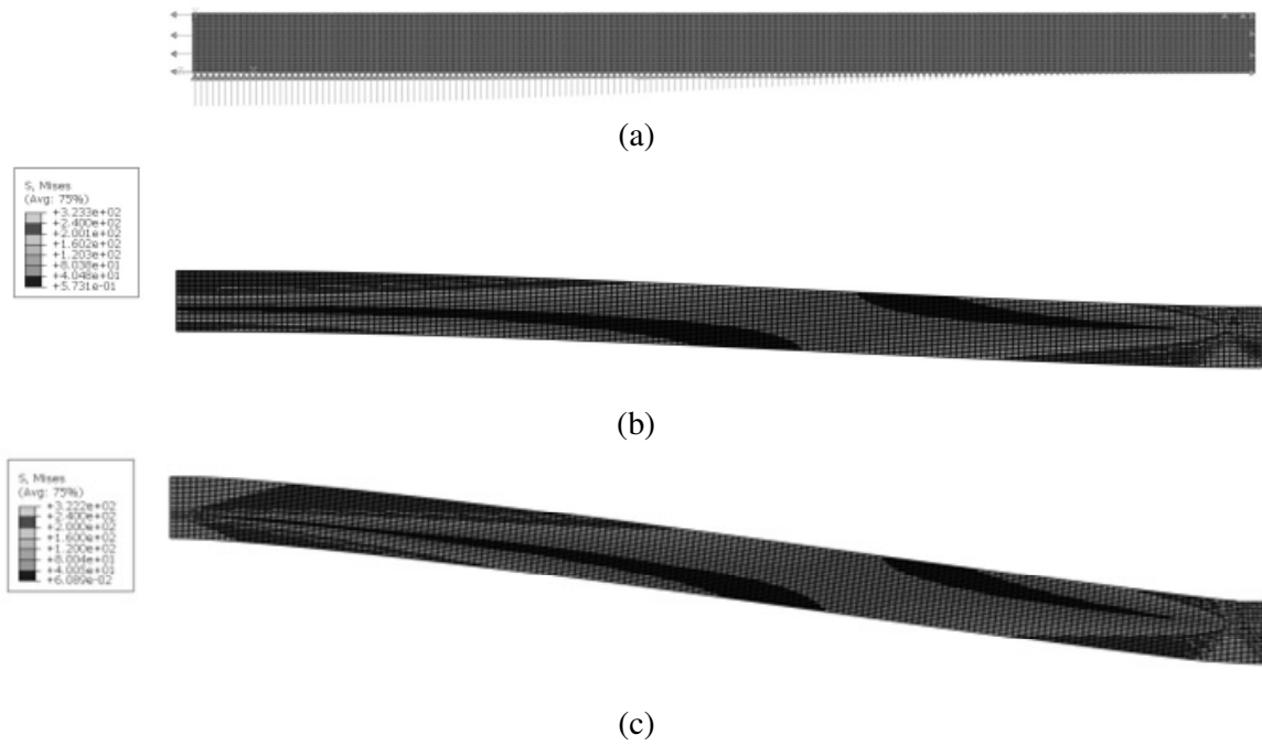
Figure 9. ABAQUS-FEM2 comparison analyses. Axial force ( \nu = 1/4 ). Mesh composed of 21x176 nodes and 3500 elements. (a) mesh and loads distributions; (b) deformed shape and Von Mises stresses at yielding ( p = 0.82 MPa ); (c) deformed shape for p = 0.96 MPa.
