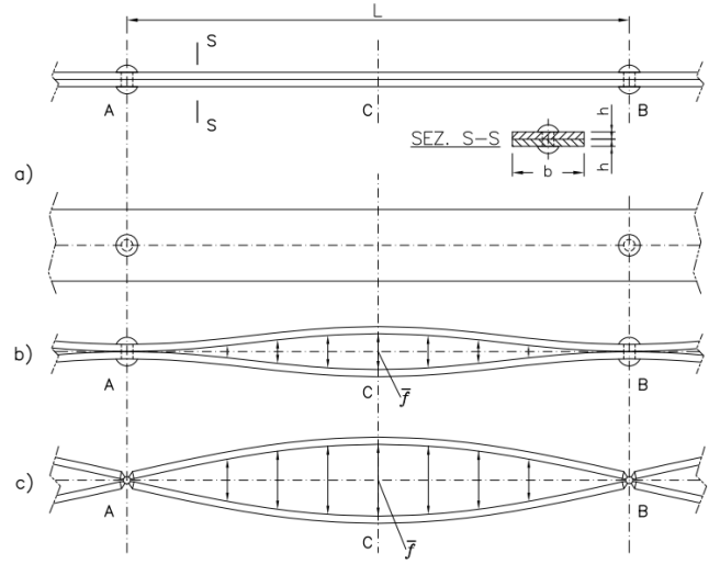
Figure 2. Tied bar composed by two rectangular rods, riveted at a pitch L . (a) undeformed configuration; (b) deformed shape A (cosinusoidal) (c) deformed shape B (sinusoidal).
