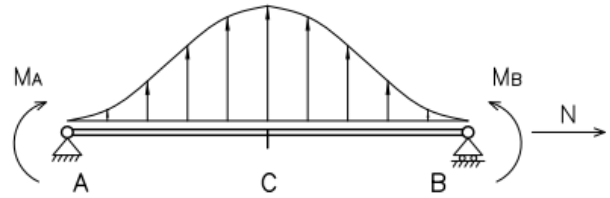
Figure 3. Simply supported beam subjected to cosinusoidal pressure profile and to plastic moment applied at the ends.
