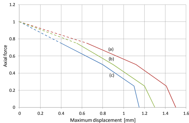
Figure 10. Relationships between axial force and maximum displacement for: (a) cosinusoidal pressure profile; (b) F.E. solution without section reduction due to the rivets hole; (c) F.E. solution with section reduction due to rivets hole.
