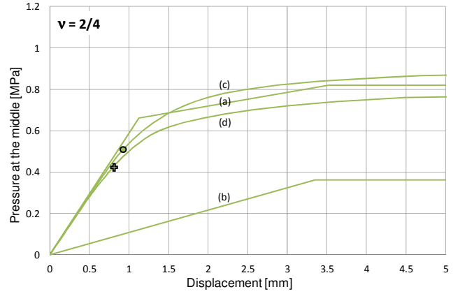
Figure 7. Pressure displacement relationships for \nu = 2/4 . Solutions for: (a) cosinusoidal pressure profile; (b) sinusoidal pressure profiles; (c) F.E. solution without section reduction due to the rivet hole; (d) F.E. solution with section reduction due to rivet hole.
