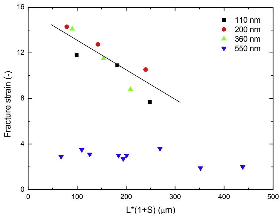
Fig. 9. Variation of the fracture strain as a function of L(1 + S) , where S is the stiffness ratio k/k_{act} . The continuous line is guide for eyes.
