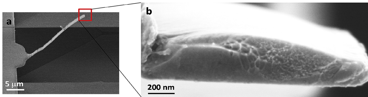
Fig. 7. Fracture surface of a beam with a thickness equal to 360 nm, showing a mirror-like surface followed by corrugations.
