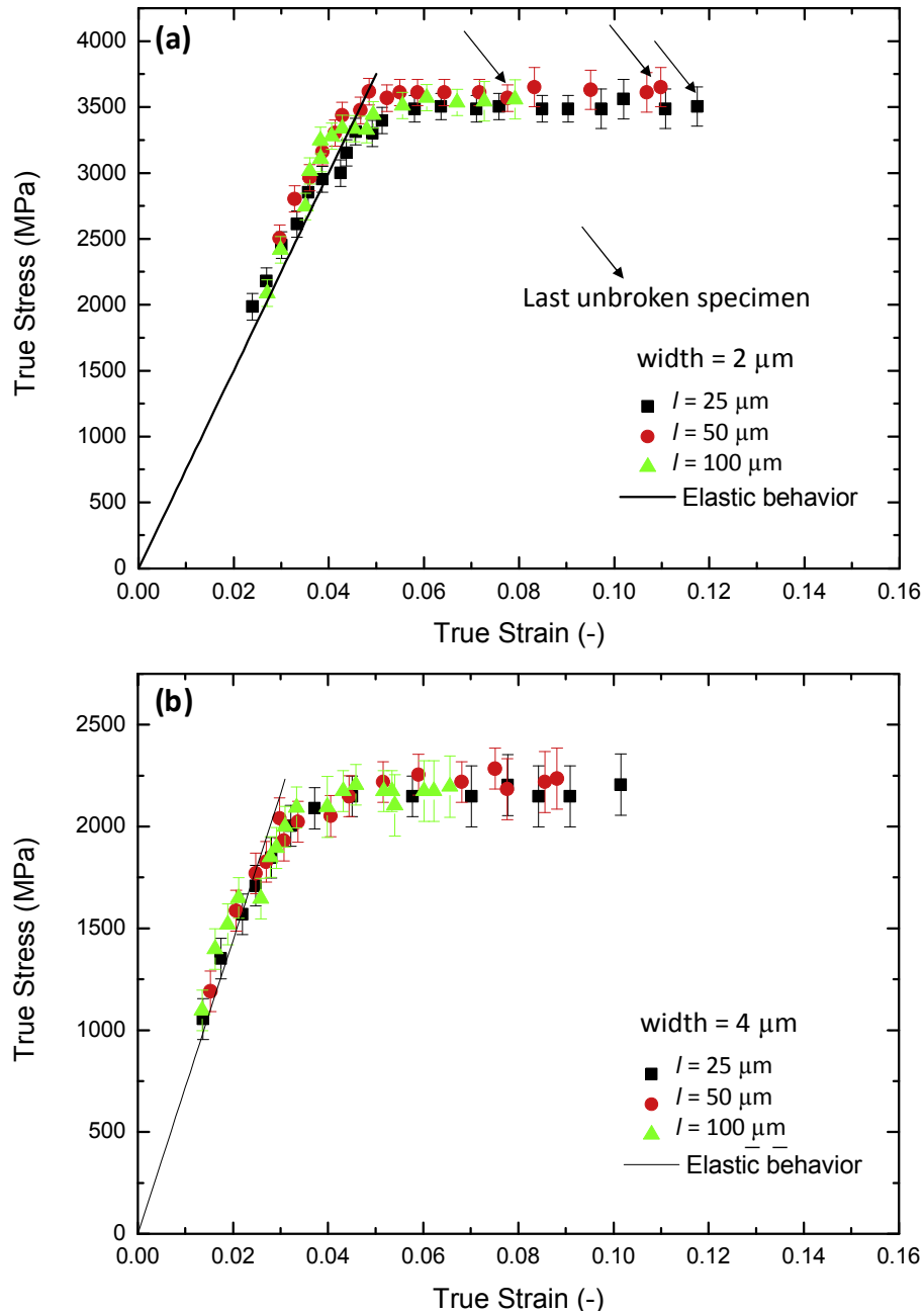
Fig. 5. True stress - true strain curves of 110 nm-thick specimens with different widths equal to 2 and 4 \mu\text{m} , respectively (a) and (b), and different lengths of 25, 50 and 100 \mu\text{m} .
