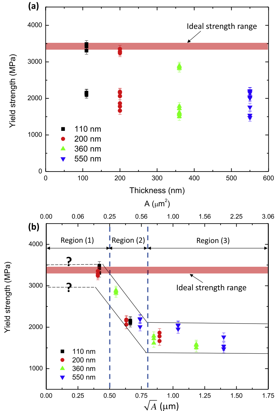
Fig. 8. (a) Variation of the yield strength as a function of the thickness; (b) variation of the yield strength as a function of the cross-sectional area and of the square root of the cross-sectional. An assumed variation of the data (eye guide) is reported and the three deformation regimes are highlighted.
