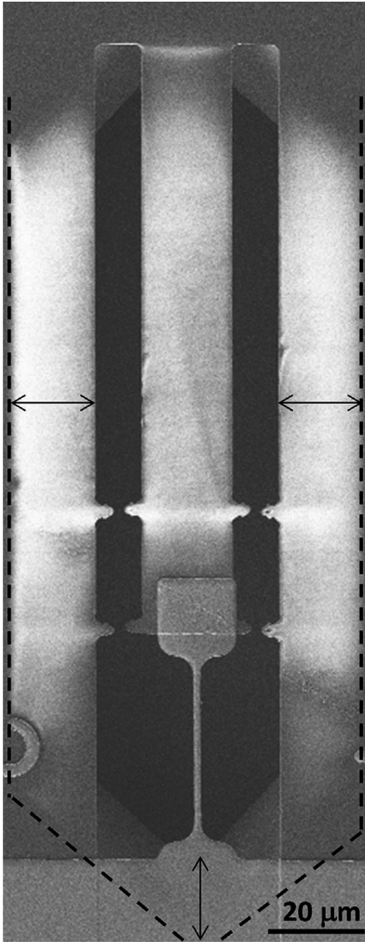
Fig. A1. SEM micrograph of a lab-on-chip highlighting the underetching corresponding to the size of the brighter zones as indicated by horizontal and vertical arrows.
