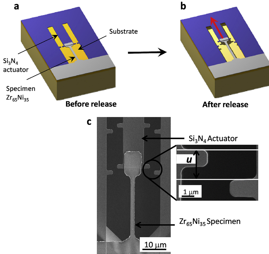
Fig. 1. The lab-on-chip method used to determine the stress-strain response; (a,b), schematic of the lab-on-chip before and after release. (c), SEM image of a deformed 25 \mu\text{m} \times 2 \mu\text{m} \times 110 \text{ nm} freestanding specimen.
