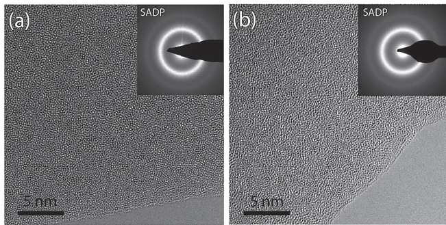
Fig. 6. Cs corrected HRTEM image on (a) as-deposited and (b) 12% deformed \text{Zr}_{65}\text{Ni}_{35} TFMGs. SAED patterns obtained with a \sim 700 nm selected area aperture are shown in the upper right insets. A fully amorphous structure is observed before and after deformation. Shear bands have not been detected in the deformed films.
