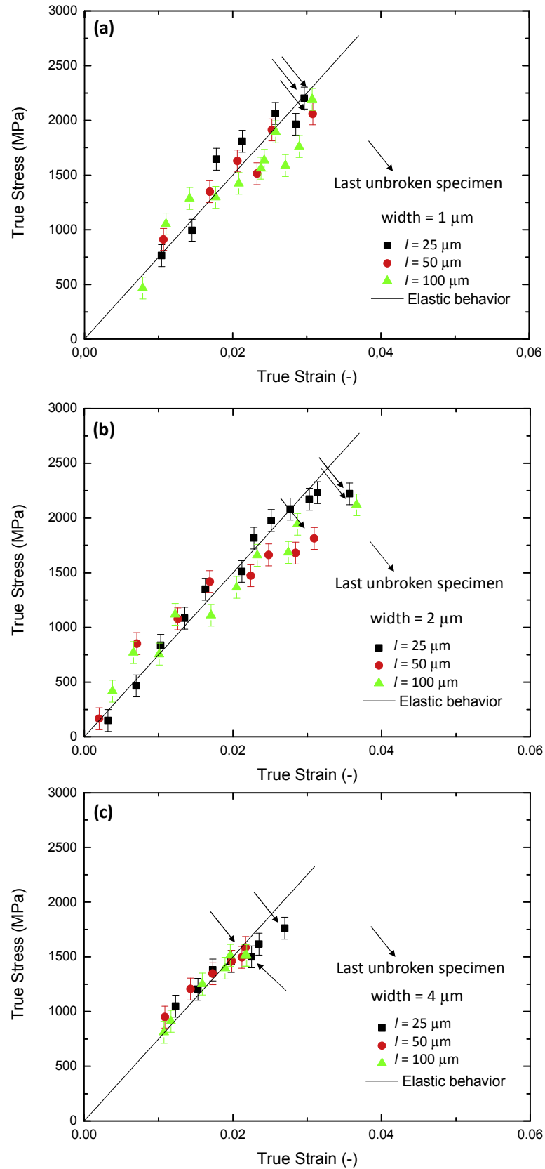
Fig. 2. True stress - true strain curves of 550 nm-thick specimens with different widths equal to 1, 2 and 4 \mu\text{m} , respectively (a), (b) and (c), and different lengths of 25, 50 and 100 \mu\text{m} .
