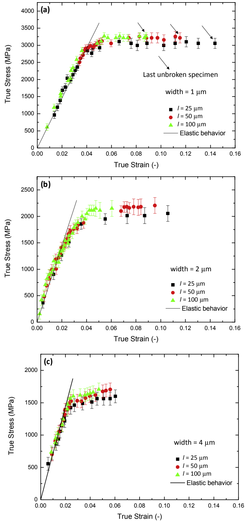
Fig. 3. True stress - true strain curves of 360 nm-thick specimens with different widths equal to 1, 2 and 4 \mu\text{m} , respectively (a), (b) and (c), and different lengths of 25, 50 and 100 \mu\text{m} .
