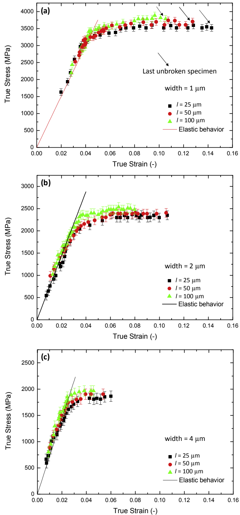
Fig. 4. True stress - true strain curves of 200 nm-thick specimens with different widths equal to 1, 2 and 4 \mu\text{m} , respectively (a), (b) and (c), and different lengths of 25, 50 and 100 \mu\text{m} .
