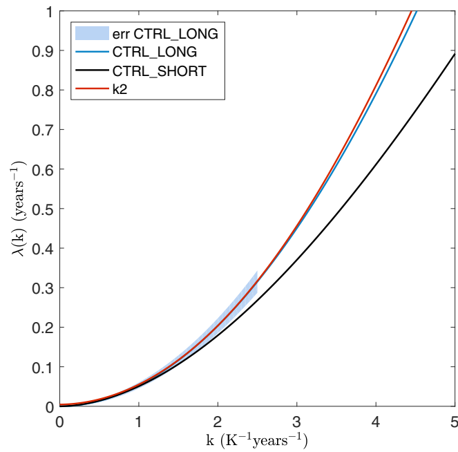
Fig. S1. The scaled cumulant generating function \lambda(k) estimated from the large deviation algorithm with k = 2 at a numerical cost of 248 y (red line) is at least as good as the one estimated from a control run lasting 1,000 y (blue line) and is much better than the one estimated from a control run lasting 248 y (black line). The shaded area corresponds to 1 SD related to the empirical average.
