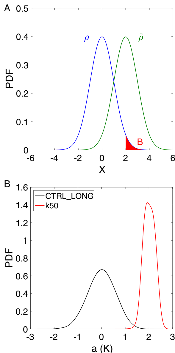
Fig. 3. (A) We want to estimate the probability to be in the set B , for the model PDF \rho(x) . We are able to sample instead from the PDF \tilde{\rho}(x) for which the rare event becomes common. We know the relation L = \rho/\tilde{\rho} and can recover the model statistics \rho , from the importance sampling \tilde{\rho} . (B) PDF of the time-averaged temperature a ( T = 90 d) for the model control run (black) and for the algorithm statistics with k = 50 , illustrating that the algorithm performs importance sampling and that +2 K heat waves become common for the algorithm while they are rare for the model.
