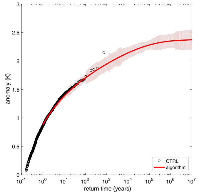
Fig. 4. Return times for the 90-d Europe surface temperature, computed from the 1,000-y-long control run (black) and from the large deviation algorithm, at the same computational cost as the control run (red). This illustrates both the good overlap on the 10- to 300-y range and the fact that the algorithm can predict probability for events that cannot be observed in the control run.
