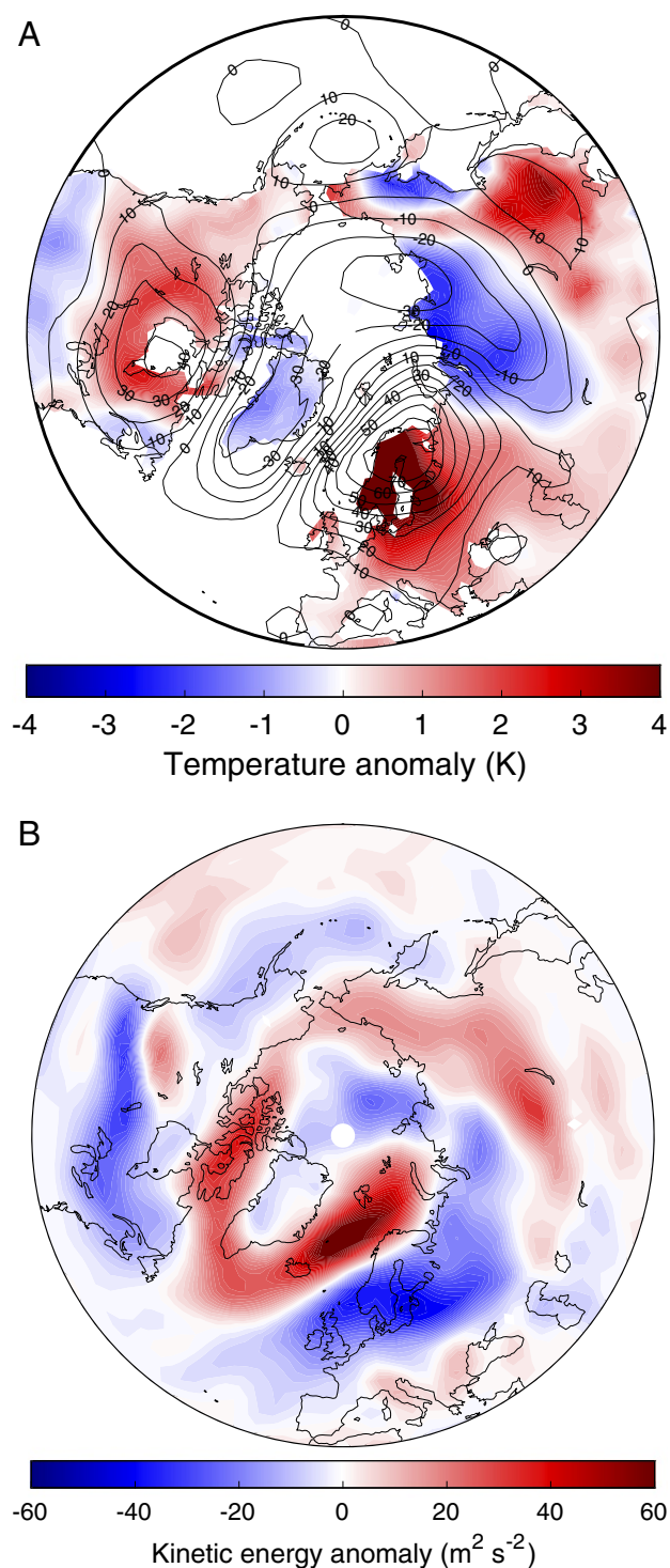
Fig. 5. (A) Northern Hemisphere surface temperature anomaly (colors) and 500-hPa geopotential height anomaly (contours), conditional on the occurrence of heat wave conditions \frac{1}{T} \int_0^T A(x_n(t)) dt > a , with T = 90 d and a = 2 K, estimated from the large deviation algorithm. (B) Northern Hemisphere anomaly of the averaged kinetic energy for the zonal velocity at 500 hPa conditional on the occurrence of heat wave conditions \mathbb{E} [KE_{500} | \frac{1}{T} \int_0^T A(x_n(t)) dt > a] , with T = 90 d and a = 2 K, estimated from the large deviation algorithm, with respect to the long-time average \mathbb{E} [KE_{500}] computed from the control run.
