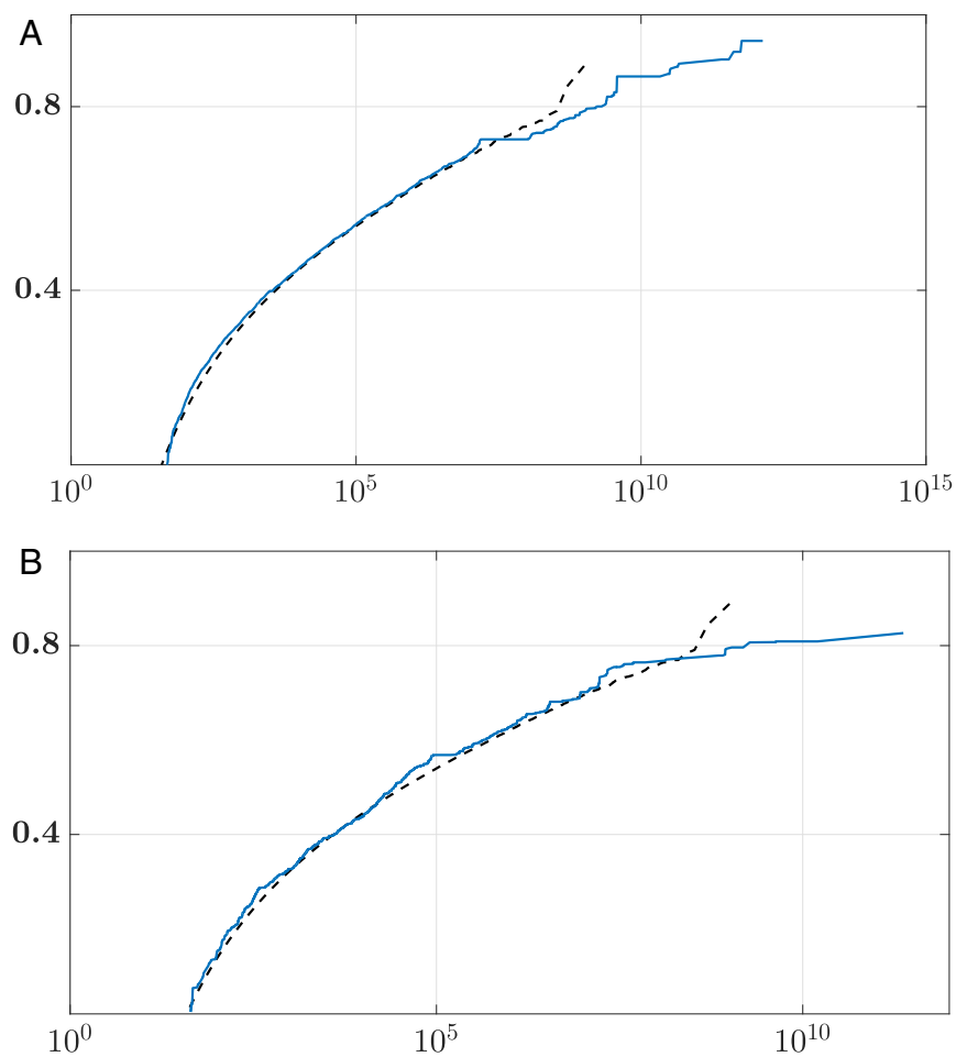
Fig. S2. Amplitude vs. return times for the Ornstein-Uhlenbeck process, from a long control run (black dashed line) and the large deviation algorithm (solid blue curve). In A , 100 algorithm realizations have been used for a total cost 160 times smaller than for the control run. In B , 10 algorithm realizations have been used for a total cost 1,600 times smaller than for the control run.
