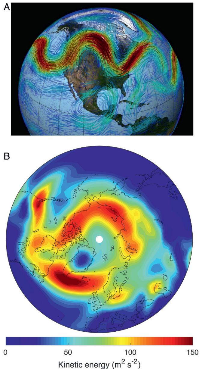
Fig. 1. (A) Snapshot of wind speed velocity at the top of the troposphere, showing the jet stream over North America (image courtesy of NASA/Goddard Space Flight Center Scientific Visualization Studio). (B) Average horizontal kinetic energy at 500 hPa (midtroposphere) in the Plasim model, showing the averaged Northern Hemisphere jet stream.
