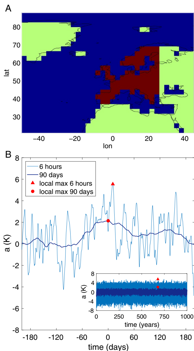
Fig. 2. (A) The red color marks the area of Europe over which the temperature is averaged. (B) Time series of European surface temperature anomaly, 6 h (light blue) and 90 d running mean (dark blue), during 360 d and 1,000 y (Inset). The red triangles and circles feature one local maximum of the temperature anomalies, as an example of a 2 K heat wave lasting 90 d.
