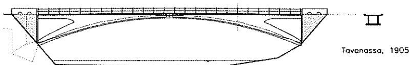
Figure 1: Robert Maillart's Tavanasa three-hinged arch bridge, 1:750
