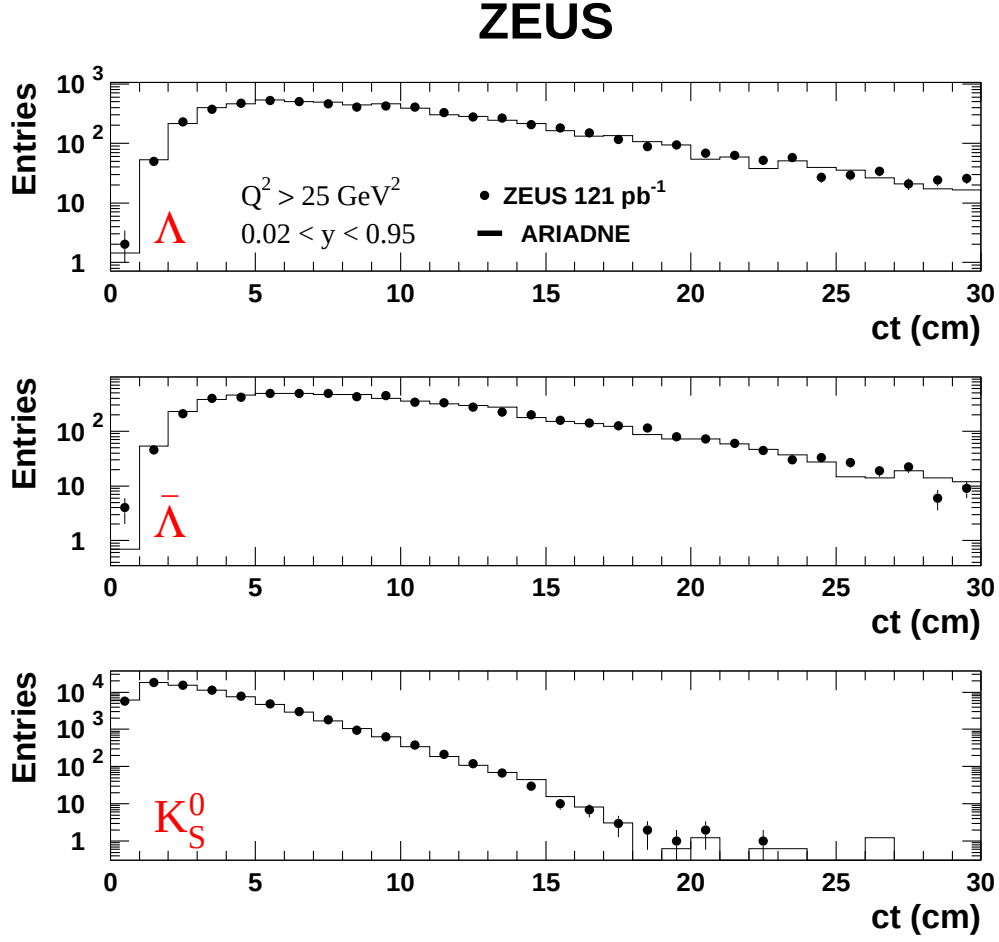
Figure 2: Detector-level distributions of ct , where t is the reconstructed proper lifetime, for \Lambda , \bar{\Lambda} and K_S^0 samples for data and ARIADNE. The ARIADNE histogram is normalised to the same number of events as the data. Statistical errors are shown unless smaller than the point size.
