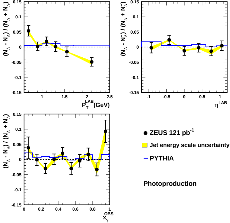
Figure 10: The ratio \frac{N(\Lambda) - N(\bar{\Lambda})}{N(\Lambda) + N(\bar{\Lambda})} as a function of P_T^{\text{LAB}} , \eta^{\text{LAB}} and x_\gamma^{\text{OBS}} , in the range 0.6 < P_T^{\text{LAB}} < 2.5 \text{ GeV} and |\eta^{\text{LAB}}| < 1.2 for events with Q^2 < 1 \text{ GeV}^2 , 0.2 < y < 0.85 and at least two jets both satisfying E_T^{\text{jet}} > 5 \text{ GeV} and |\eta^{\text{jet}}| < 2.4 . Statistical errors are shown, together with the uncertainty arising from the jet energy scale (shaded band). The solid histogram shows the prediction from PYTHIA (with multiple interactions).
