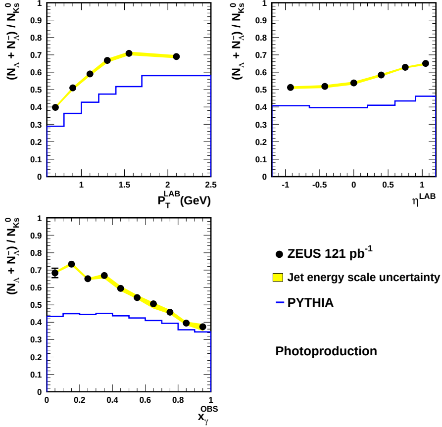
Figure 15: The ratio \frac{N(\Lambda) + N(\bar{\Lambda})}{N(K_S^0)} as a function of P_T^{\text{LAB}} , \eta^{\text{LAB}} and x_{\gamma}^{\text{OBS}} , in the range 0.6 < P_T^{\text{LAB}} < 2.5 \text{ GeV} and |\eta^{\text{LAB}}| < 1.2 for events with Q^2 < 1 \text{ GeV}^2 , 0.2 < y < 0.85 and at least two jets both satisfying E_T^{\text{jet}} > 5 \text{ GeV} and |\eta^{\text{jet}}| < 2.4 . The statistical errors are shown, unless smaller than the point size. The shaded band shows the uncertainty arising from the jet energy scale. The solid histogram shows the prediction from PYTHIA (with multiple interactions).
