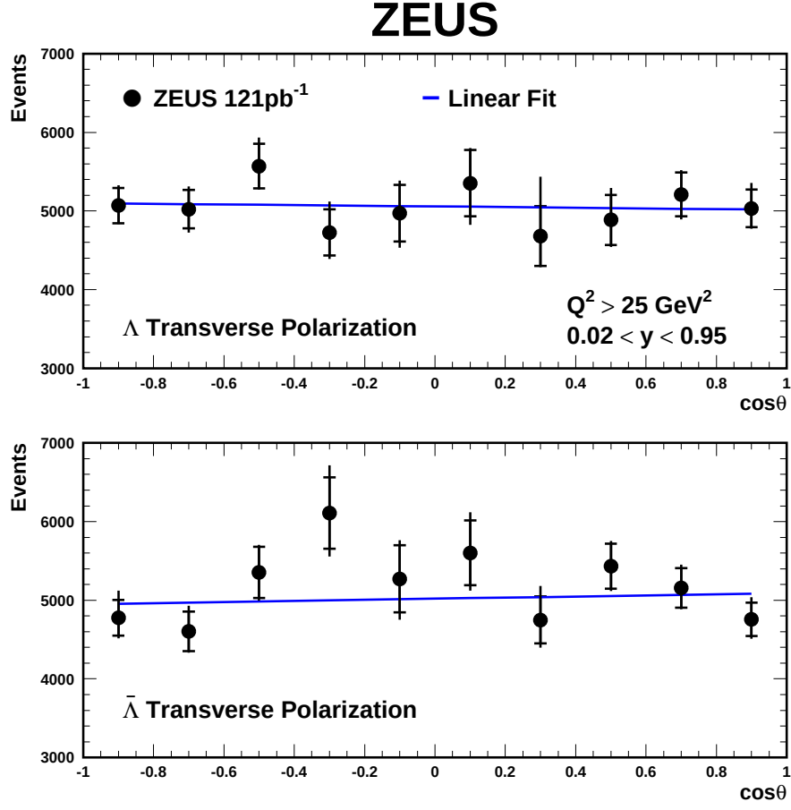
Figure 20: Angular distributions of the highest-momentum decay particle from a \Lambda or \bar{\Lambda} in the range 0.6 < P_T^{\text{LAB}} < 2.5 \text{ GeV} and |\eta^{\text{LAB}}| < 1.2 for events with Q^2 > 25 \text{ GeV}^2 and 0.02 < y < 0.95 , where \theta is the angle between the decay-particle momentum vector and the polarization axis, in the rest frame of the \Lambda or \bar{\Lambda} . Statistical errors (inner error bars) and the systematic uncertainties added in quadrature are shown. The first-order polynomial fit (solid line) from which the polarization is obtained is also shown.
