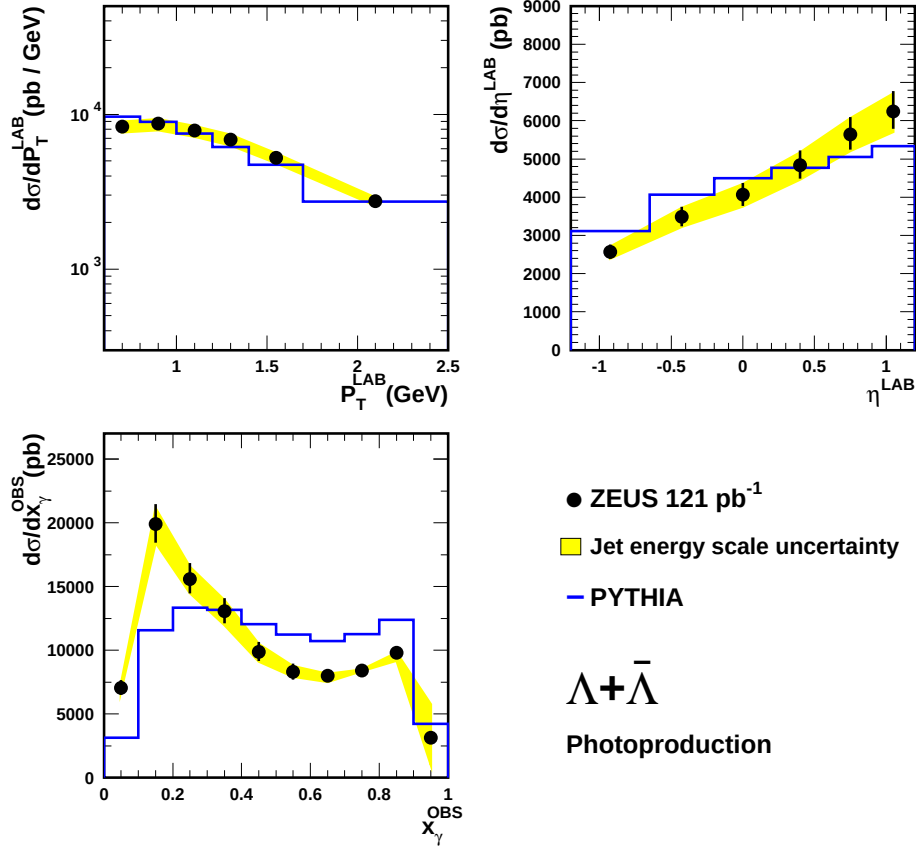
Figure 8: Differential \Lambda + \bar{\Lambda} cross sections as a function of P_T^{\text{LAB}} , \eta^{\text{LAB}} and x_\gamma^{\text{OBS}} , in the range 0.6 < P_T^{\text{LAB}} < 2.5 \text{ GeV} and |\eta^{\text{LAB}}| < 1.2 for events with Q^2 < 1 \text{ GeV}^2 , 0.2 < y < 0.85 and at least two jets both satisfying E_T^{\text{jet}} > 5 \text{ GeV} and |\eta^{\text{jet}}| < 2.4 . Statistical errors are shown, unless smaller than the point size, together with the systematic uncertainty arising from the trigger efficiency added in quadrature. The uncertainty arising from the jet energy scale is also shown (shaded band). The solid histogram shows the prediction from PYTHIA (with multiple interactions), normalised to the data.
