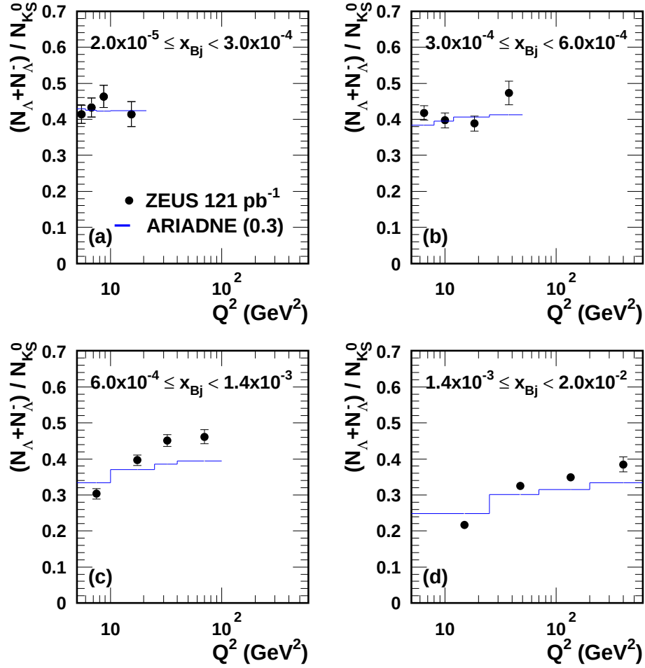
Figure 13: The ratio \frac{N(\Lambda) + N(\bar{\Lambda})}{N(K_S^0)} as a function of Q^2 for four bins of x_{Bj} , in the range 0.6 < P_T^{\text{LAB}} < 2.5 GeV and |\eta^{\text{LAB}}| < 1.2 for events with Q^2 > 5 GeV 2 and 0.02 < y < 0.95 . Statistical errors only are shown. The histograms show predictions from ARIADNE with a strangeness-suppression factor of 0.3.
