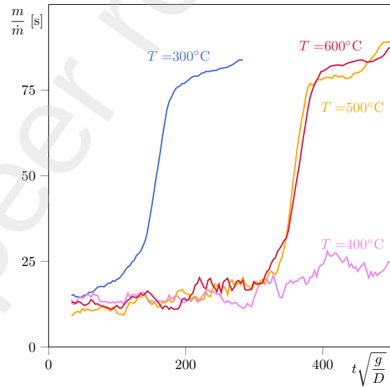
Figure 16: Droplet instantaneous lifetime.
