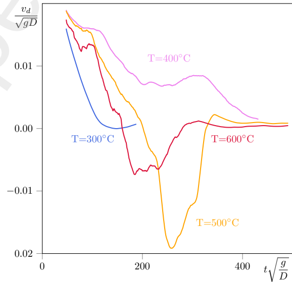
Figure 14: Droplet velocity evolution
