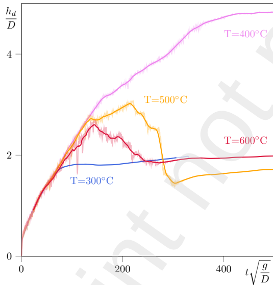
Figure 13: Droplet depth evolution
