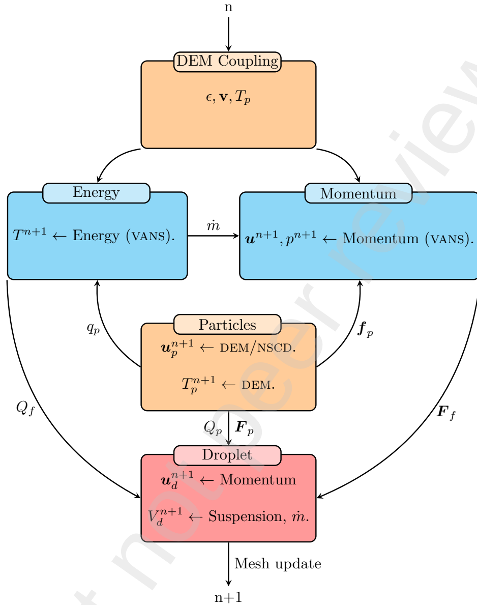
Figure 11: Numerical procedure.
