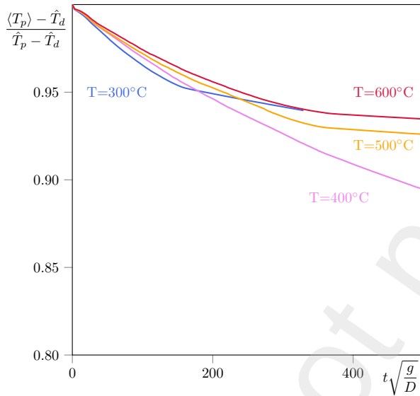
Figure 15: Mean particle temperature evolution.
