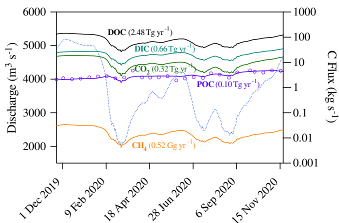
Fig. 6. LOADEST modeled instantaneous downstream fluxes of DOC (black), DIC (light blue), CO 2 (green), POC (purple), and CH 4 (orange). Calculated POC fluxes (discharge × concentration) are shown as purple circles. Total annual flux of each C species is shown in parentheses. Discharge is shown as a dotted blue line.
