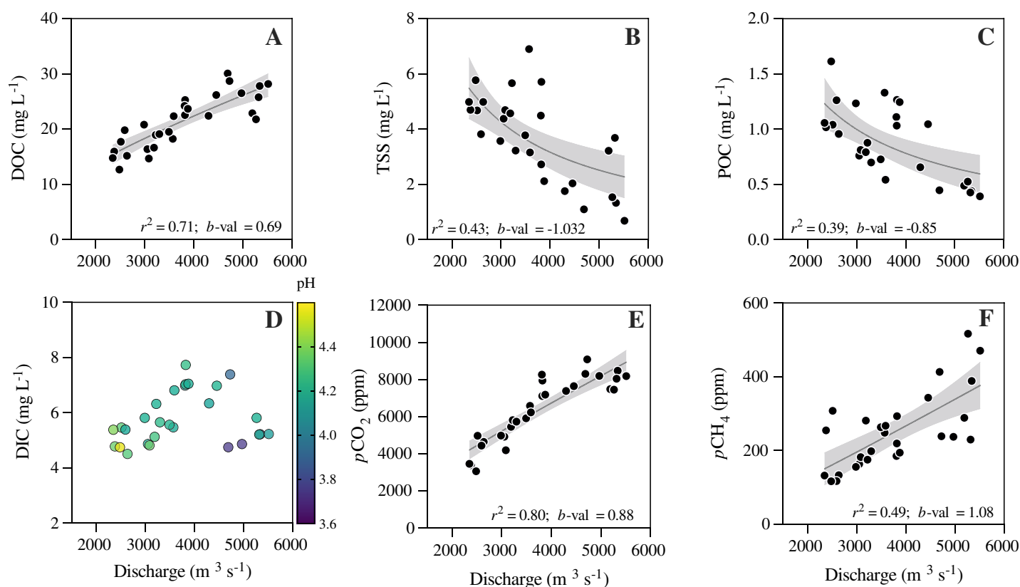
Fig. 4. DOC (A), total suspended sediment (B), POC (C), DIC (D), pCO 2 (E), and pCH 4 (F) correlated with discharge. Power regressions (gray line) are shown with 95% confidence intervals (light gray bands).
