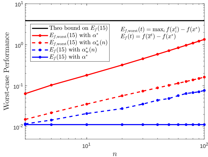
Figure 1 Comparison of the average functional error E_f (53) and the worst functional error E_{f,\text{worst}} (54) for t = 15 iterations of the EXTRA algorithm and their evolution with the number of agents n in the system. The plot shows (i) the constant theoretical bound on E_f (51), in black, (ii) the PEP bounds on the function error of the worst agent E_{f,\text{worst}} , scaling sublinearly with n , in red and (iii) the PEP bounds for the function error of the average iterate E_f , in blue. The constant step-size \alpha^* has been optimized for this performance criterion and leads to a bound constant with n (plain blue line). Step-sizes can also be optimized with respect to E_{f,\text{worst}}(15) , leading to smaller step-sizes \alpha_w^*(n) decreasing as \frac{1}{\sqrt{n}} . They improve the guarantee for E_{f,\text{worst}} and its scaling with n but they deteriorate the corresponding guarantee for E_f (see dashed lines). In this plot, the range of eigenvalues for the averaging matrix is [-0.5, 0.5] and the local functions are 1-smooth and 0.1-strongly convex.
