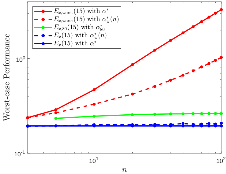
Figure 2 Comparison of the average iterates error E_x (53), the worst iterates error E_{x,\text{worst}} (54) and the 80-th percentile iterates error E_{x,80} (55) for t = 15 iterations of the EXTRA algorithm and their evolution with the number of agents n in the system. The plot shows (i) the PEP bounds on the iterates error of the worst agent E_{x,\text{worst}} , scaling sublinearly with n , in red, (ii) the PEP bound on the 80-th percentile iterates error E_{x,80} , in green, and (iii) the PEP bounds for the average iterates error E_x , in blue. The constant step-size \alpha^* has been hand-tuned for this performance criterion and leads to a bound constant with n (plain blue line). Step-sizes can also be hand-tuned with respect to E_{f,\text{worst}}(15) , leading to smaller step-sizes \alpha_w^*(n) . They improve the guarantee for E_{f,\text{worst}} and its scaling with n without deteriorating too much the corresponding guarantee for E_f (see dashed lines). In this plot, the range of eigenvalues for the averaging matrix is [-0.5, 0.5] and the local functions are 1-smooth and 0.1-strongly convex.
