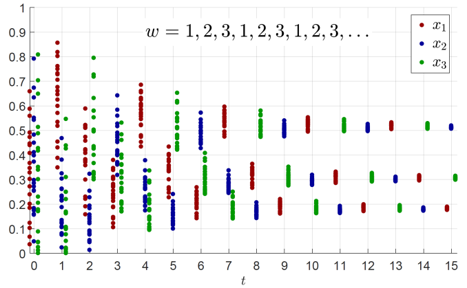
Fig. 4. Trajectories from different initial conditions x = [x_1, x_2, x_3]^\top , for a periodic signal w = \{1, 2, 3, 1, 2, 3, 1, 2, 3, \dots\} \in \mathcal{L} . All trajectories quickly converge to the same orbit, as predicted by 1-dominance.
