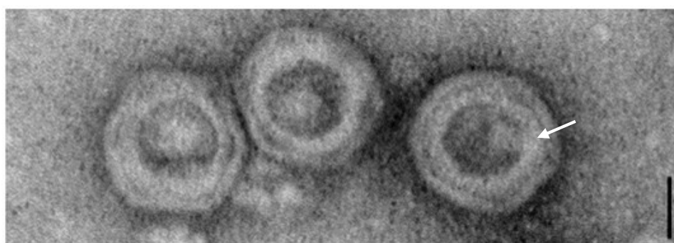
Figure 6. Transmission electron micrograph of phage Wip1 particles negatively stained with 2% uranyl acetate. Phage Wip1 has the typical tail-less isometric heads of Tectiviridae with an internal lipid membrane (highlighted by the arrow). Scale bar represents 25 nm. Reproduced from Schuch et al. (2009), PLoS One (reference [180]).
