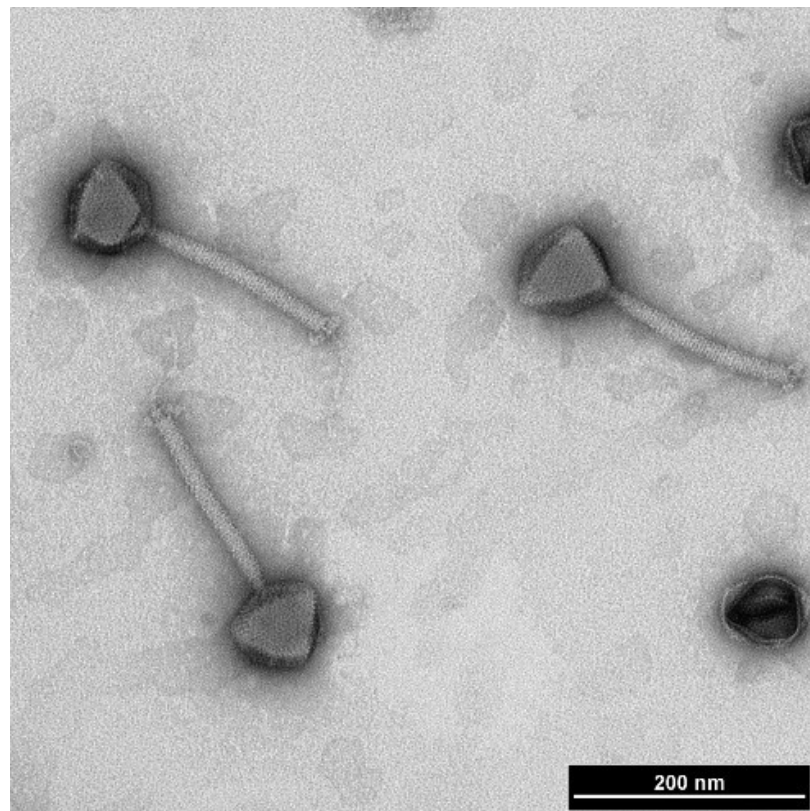
Figure 2. Transmission electron micrograph of the Twort-like phage vB_BceM_Bc431v3. Phage particles display isometric heads 85.4 \pm 3 nm in diameter with individual capsomers. The phage possesses a long contractile tail 180 \pm 3 nm in length by 12 \pm 4 nm in width. Reproduced from El-Arabi et al. (2013), Virol. J. (reference [68]).
