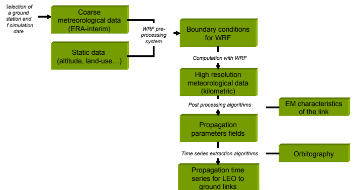
Figure 1: Flow chart of the simulator
