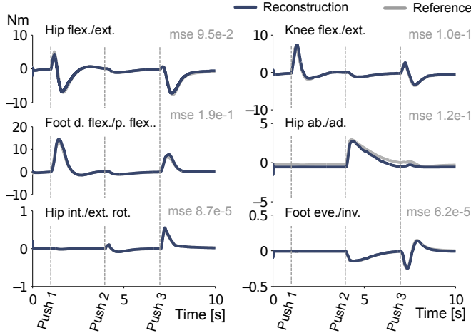
Fig. 7. The reconstructed torques (dark blue) approximate with high accuracy the reference torques (grey).
