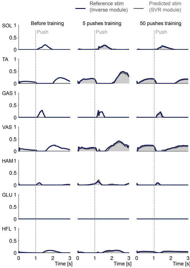
Fig. 8. Evolution of the predicted muscular stimulations at different learning stages for the same forward push, in the sagittal plane and on the torso (10N). The robot is trained with random magnitude pushes in the sagittal plane.
