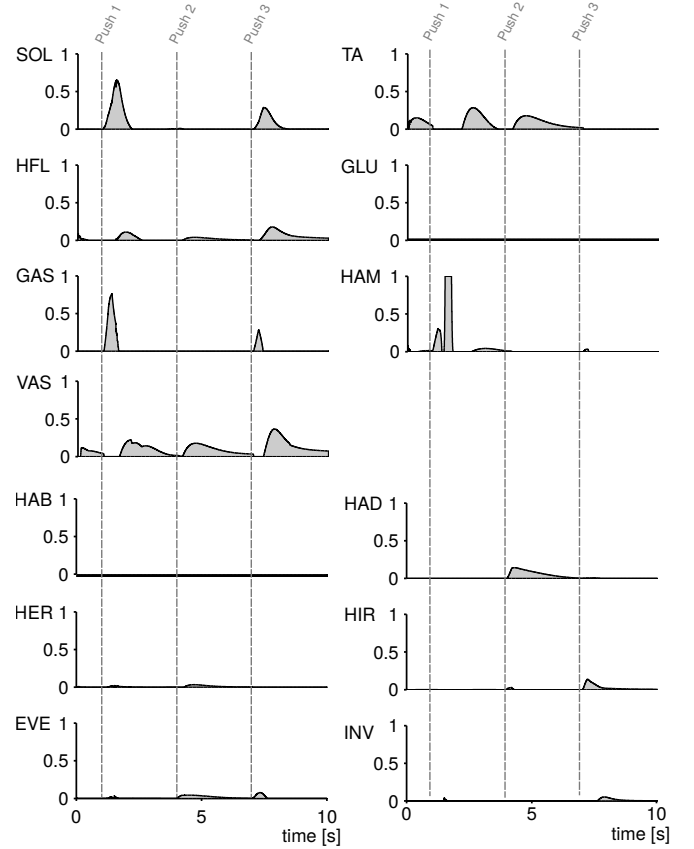
Fig. 6. Muscular stimulations for all 13 muscles generated by the inverse muscle model when the robot is receiving the benchmark perturbations.
