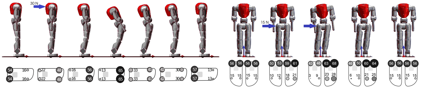
Fig. 5. Recovery motion for a horizontal perturbation on the torso (sagittal plane) and a horizontal perturbation on the waist (frontal plane). The lower panels show the evolution of the contact forces (in N) during the recovery motion.
