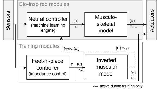
Fig. 1. Architecture of the main controller. Based on the sensed perturbation, the neural controller generates muscular stimulations (a) to drive a musculoskeletal model. The resulting joint torques (b) actuate the robot lower limbs. In parallel, an impedance controller computes desired torques (c) being transformed into virtual stimulations (d) by an inverse muscular model. These are used by the neural controller during the learning phase. The impedance controller further computes the upper-limb reaction torques (e), for which no muscular model was developed.
