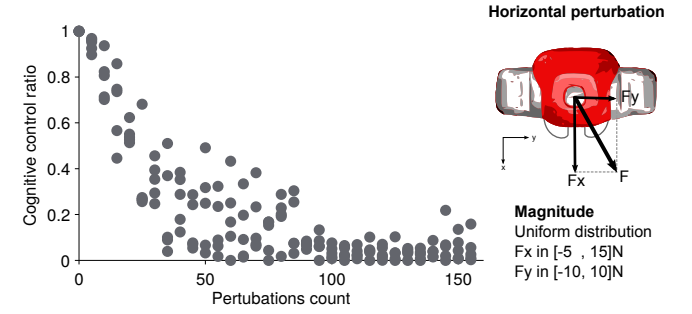
Fig. 10. Using SVR, the cognitive control ratio decreases as more training data becomes available. The figure overlays five runs while delivering perturbations in the whole transverse plane.
