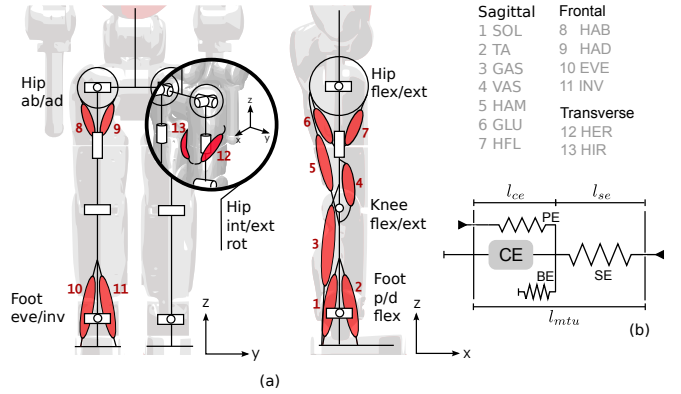
Fig. 2. (a) 3D lower limbs musculoskeletal model comprising 13 Hill-type muscles (b) per leg.
