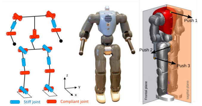
Fig. 4. COMAN: a 23 DOF compliant humanoid robot: real robot and simulation model (adapted from [3]).
