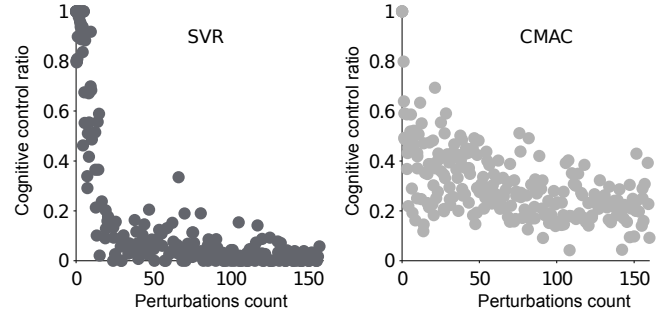
Fig. 9. The cognitive control ratio decreases as more training data becomes available. The figure overlays five runs while delivering perturbations in the sagittal plane only.
