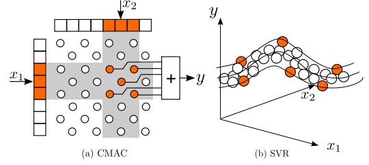
Fig. 3. (a) CMAC model: each input range is discretized. A specific multidimensional input activates a fixed number of input neurons (the orange cells of x_1 and x_2 in this figure). Based on the activated input neurons, specific core neurons are recruited. Their respective weights are summed to produce the output y . (b) SVR: some data points are elected to become support vectors.
