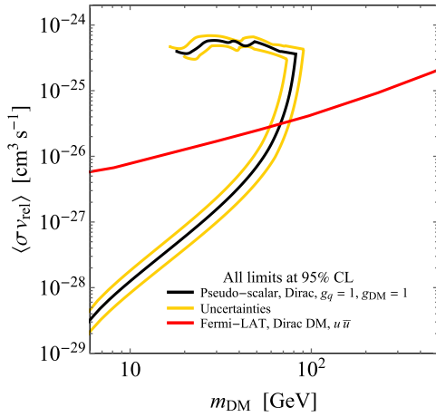
Fig. 3. A comparison of the LHC result to the Fermi-LAT limit in the m_{\text{DM}} - \langle \sigma v_{\text{rel}} \rangle plane. Both limits are at 95% CL. The Fermi-LAT limit is for Dirac DM and assumes that the only annihilation channel is to u\bar{u} quarks. The Fermi-LAT limits to other quark-anti-quark annihilation channels will be similar. The LHC exclusion contour is for a pseudo-scalar mediator, Dirac DM and couplings g_q = 1 and g_{\text{DM}} = 1 . The shown LHC results are intended for illustration only and are not based on real data.
