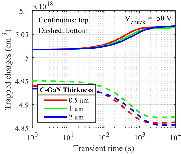
Fig. 10. Simulated evolution of top and bottom buffer charge during the stress phase ( V_{\text{chuck}} = -50 V) for different C-GaN thicknesses. [C] = 10^{19} \text{ cm}^{-3} .
