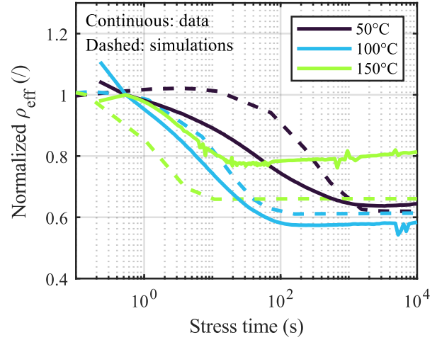
Fig. 8. Simulated and measured normalized effective resistivity during the stress phase ( V_{\text{chuck}} = +50 \text{ V} ). Long time constants and temperature-dependent features observed experimentally are reproduced by the 2D TCAD model.
