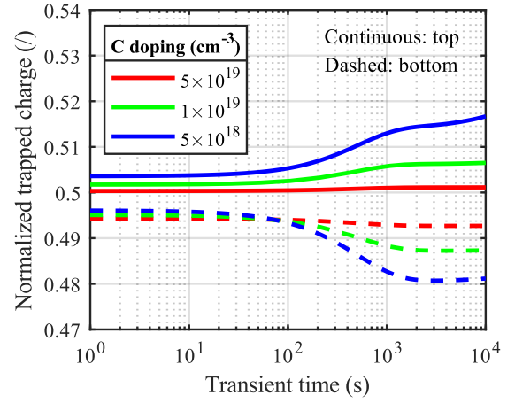
Fig. 9. Simulated evolution of trapped charge close to top and bottom interfaces of the C-doped buffer while stressing the substrate at V_{\text{chuck}} = -50 \text{ V} , for different C concentrations. The charge is normalized to the C concentration. Redistribution of charges is not significantly accelerated or slowed down by changing C doping in the buffer.
