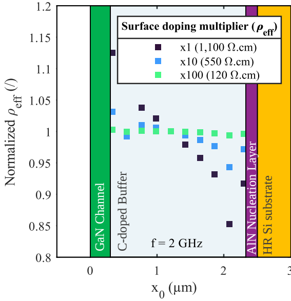
Fig. 7. Variation of normalized \rho_{\text{eff}} as a function of the position of the localized charge (peak density: 3 \times 10^{17} \text{ cm}^{-3} ) for three different substrates showing typical \rho_{\text{eff}} values. The relative variation is strongest for the substrate showing highest \rho_{\text{eff}} .
