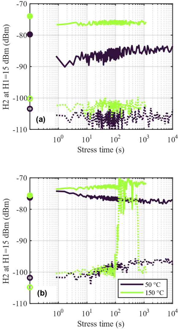
Fig. 4. Experimental variation of 2 nd (continuous) and 3 rd (dotted) harmonic power at the output of 2 mm-long CPW lines of sample A while stressing the chuck at (a) -50 V and (b) +50 V. Because measurement acquisition time is larger for HD measurement compared with S-parameters, the experimental time resolution is only of ~1 s. Symbols indicate the pre-stress measurement.
