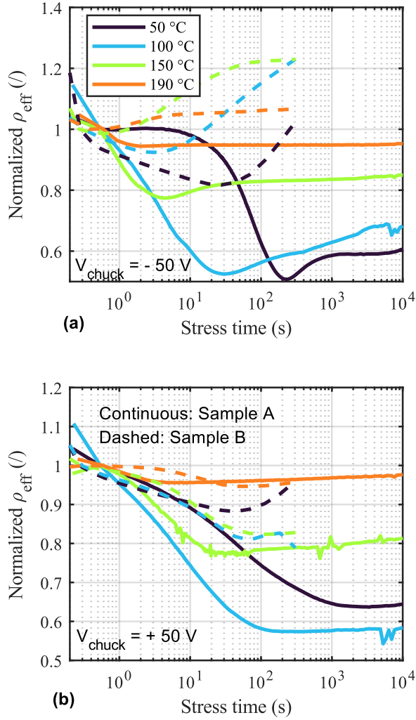
Fig. 3. Experimental stress sequences for the GaN-on-Si substrates considered here, for chuck temperature ranging from 50 °C to 190 °C: (a) V_{\text{chuck}} = -50 V and (b) V_{\text{chuck}} = +50 V. The data is normalized to the 2 nd measured point to remove the absolute decrease of \rho_{\text{eff}} with temperature (see [15]).
