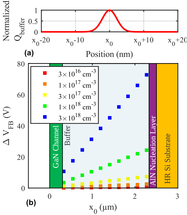
Fig. 5. (a) Charge distribution used in the simulated MIS stack. (b) Flat-band voltage shift calculated for the charge distribution shown in (a). The position of the peak charge is varied from the GaN channel/buffer interface to the buffer/AlN interface. \Delta V_{FB} depends on the charge density, but also on its position in the buffer.
