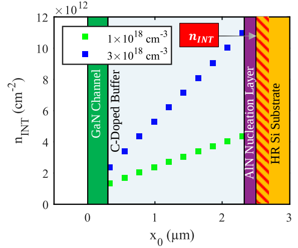
Fig. 6. Interface free carrier sheet density for different positions of the localized charge. For high peak charge, n_{INT} is strongly affected by buffer charge location.
