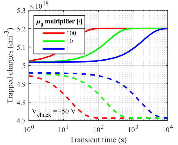
Fig. 11. Simulated evolution of top and bottom buffer charge during the stress phase ( V_{\text{chuck}} = -50 V) for varying hole mobility. Enhanced hole transport across the III-N layers can greatly reduce the time-dependence of \rho_{\text{eff}} through accelerated charge redistribution.
