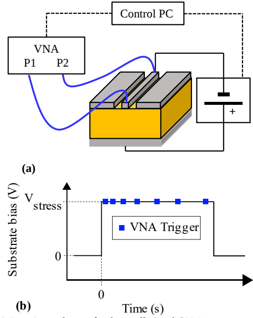
Fig. 2. (a) Experimental setup for the small-signal CPW stress measurements. For time-dependent HD measurements, a power amplifier and RF filters are added between VNA P1 and the CPW line. (b) Schematic of the measurement sequence. After substrate DC bias has been stepped to +50 V or -50 V, successive RF measurements (represented by squares) are taken on the CPW line. The relaxation phase is also represented.
