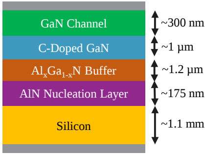
Fig. 1. Cross-sectional schematic of the studied and simulated GaN-on-Si stack. Electrodes are represented schematically in gray
