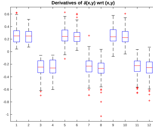
Figure 5: Nonlinear case: distributions of the partial derivatives of \delta(x, y) with respect to the p + q elements (x, y) , they are given from the left to the right by quadruples (\partial\delta(x, y)/\partial x_1, \partial\delta(x, y)/\partial x_2, \partial\delta(x, y)/\partial y_1, \partial\delta(x, y)/\partial y_2) : cases 1 to 4, pseudo-true values, cases 5 to 8, the FDH estimators and cases 9 to 12, the order- m estimators. Here n = 400 , m = 200 with p = q = 2 .
