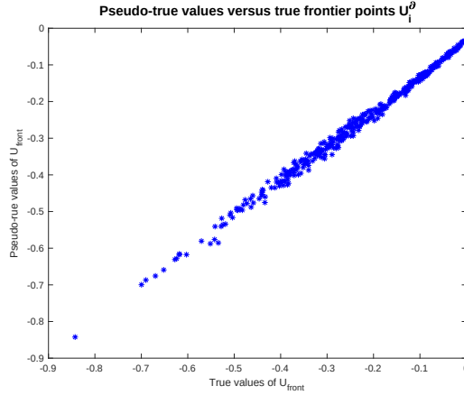
Figure 2: Nonlinear case: pseudo-true fitted values \alpha_{0,n}(V_i) versus true values U_i^\partial , n = 400 with p = q = 2 .
