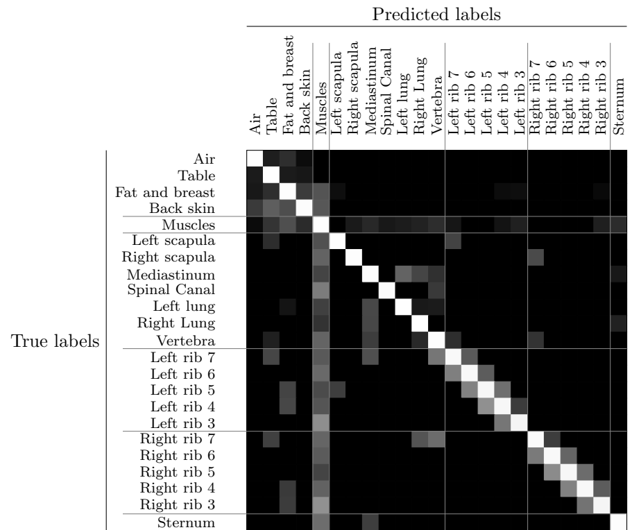
Figure D.1 – Representation of the confusion matrix. Each row was normalized so that it adds up to one. To improve visual contrast among the off-diagonal entries, the fourth root was applied. One can observe that many small portions of organs are sometimes misclassified as being muscle. Similarly, the series of numbered ribs is sometimes shifted by one position, the rib next to the vertebra being then merged with the latter.
