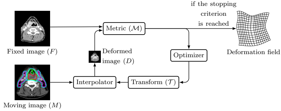
Figure 2.9 – Registration of two images. For more details, refer to the text.
