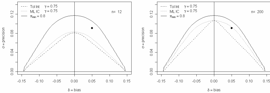
Figure 6: Iso-power line in the \delta, \sigma space of the tolerance interval and maximum likelihood validation methods for two samples sizes ( n=12 and n=200 ). The outer (solid) line delimits the true acceptance region for \pi_{\min} = 0.8 .
