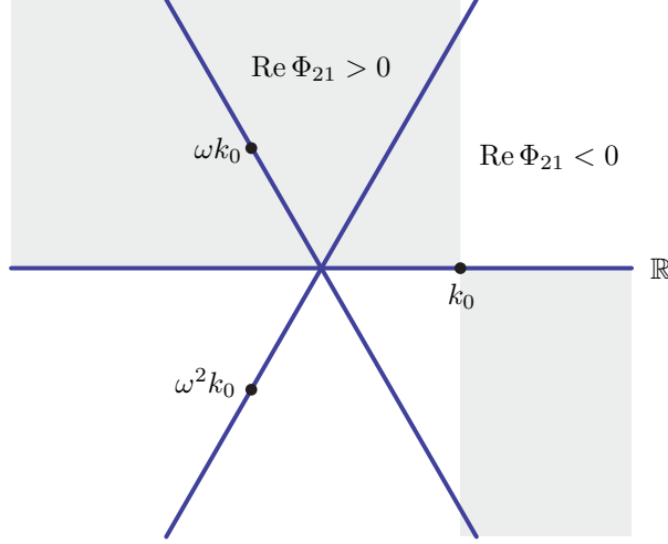
Figure 5. The regions where \operatorname{Re} \Phi_{21} > 0 (shaded) and \operatorname{Re} \Phi_{21} < 0 (white).
