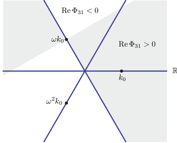
Figure 6. The regions where \operatorname{Re} \Phi_{31} > 0 (shaded) and \operatorname{Re} \Phi_{31} < 0 (white).
