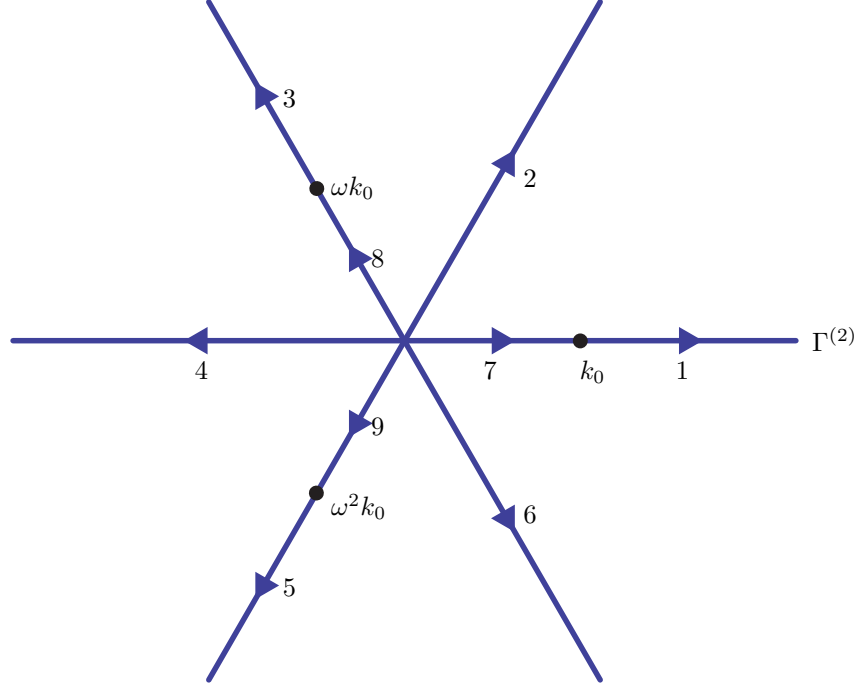
Figure 9. The contour \Gamma^{(2)} in the complex k -plane.
