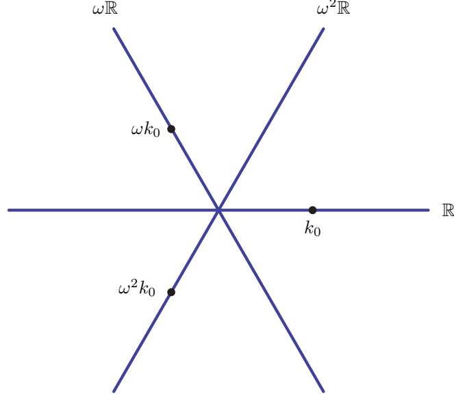
Figure 4. The three critical points k_0, \omega k_0, \omega^2 k_0 in the complex k -plane for \zeta > 0 .
