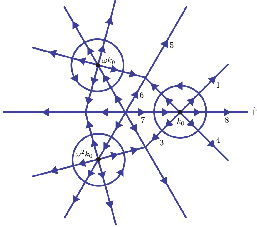
Figure 12. The contour \hat{\Gamma} = \Gamma^{(3)} \cup \partial\mathcal{D} in the complex k -plane.
