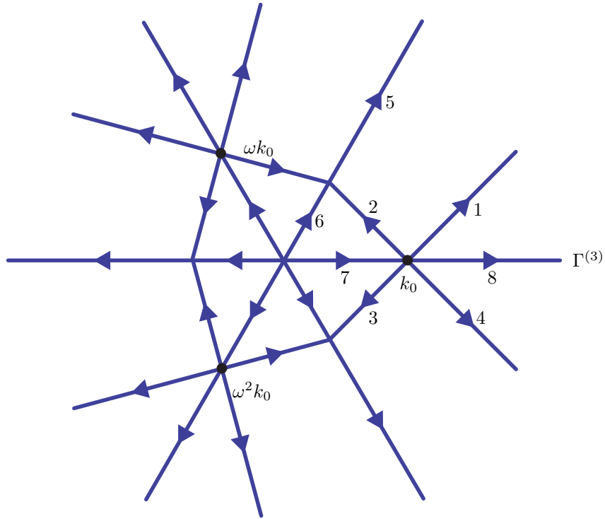
Figure 11. The contour \Gamma^{(3)} in the complex k -plane.
