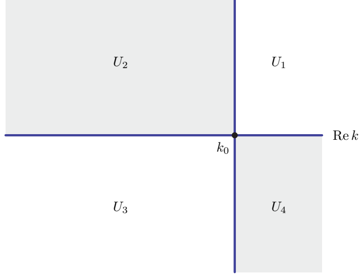
Figure 8. The open sets \{U_j\}_1^4 in the complex k -plane.
