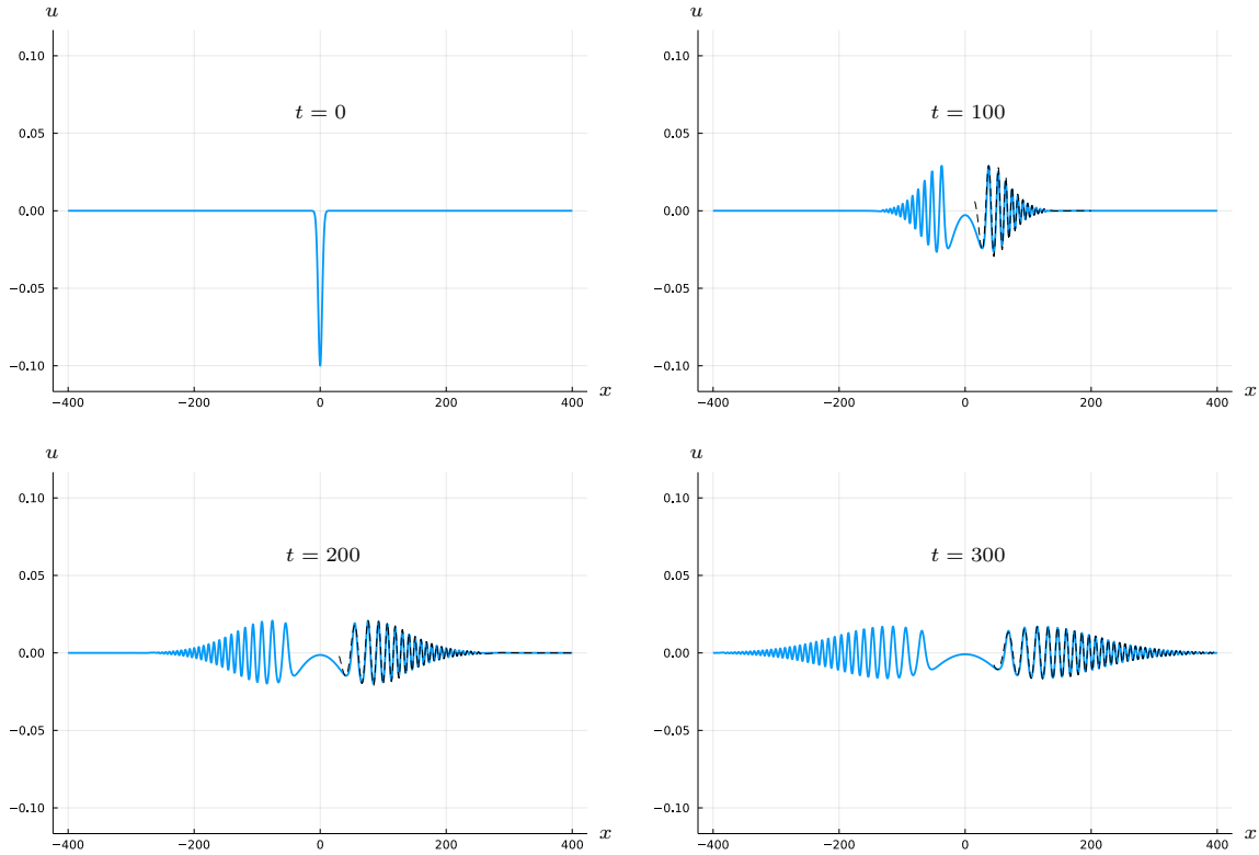
Figure 3. Numerical simulation of the solution u(x, t) of (1.4) with initial data u(x, 0) = -\frac{1}{10}e^{-x^2/20} and u_t(x, 0) = 0 (solid blue) together with the asymptotic approximation in (2.9) (dashed black) at the times t = 0 , t = 100 , t = 200 , and t = 300 . As expected, the asymptotic formula provides a better and better approximation as t increases. The convergence is the slowest for small values of x , which is consistent with the fact that the asymptotic estimate (2.9) is not uniform near x = 0 .
