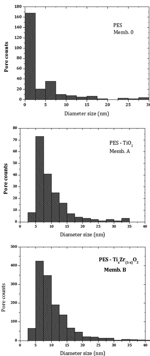
Fig. 9 Pore size distributions of PES control, PES-TiO 2 and PES-Ti x Zr (1-x) O 2 membranes.
