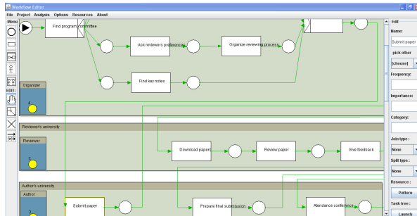
Figure 9 Workflow to organize a conference
