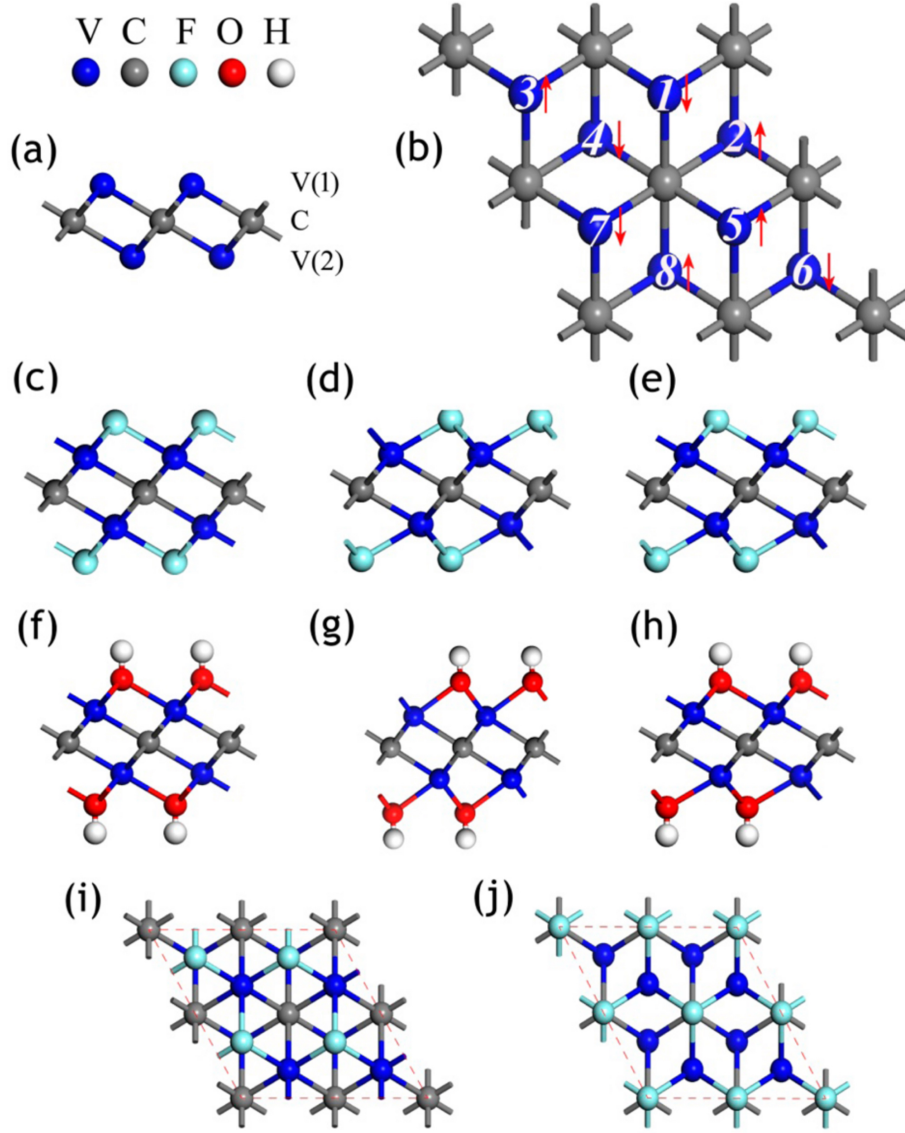
Figure 5.5: Optimized structural geometries of the free-standing V_2C monolayer and its fluorinated and hydroxylated derivatives. (a) Side view of the bare V_2C monolayer consists of a triple-layer with V(1) CV(2) stacking sequence. (b) Top view of the V_2C monolayer with T5 magnetic configuration. (c-h) Side views of (c) I- V_2CF_2 , (d) II- V_2CF_2 , (e) III-I- V_2CF_2 , (f) I- V_2COH_2 , (g) II- V_2COH_2 , and (h) III-I- V_2COH_2 . (i, j) top views of I- V_2CF_2 and II- V_2CF_2 [151].
