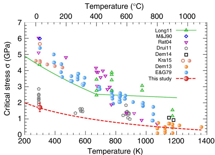
Fig. 1. Critical stress for plastic flow as a function of temperature. The red circle was obtained by including our in situ dislocation velocity measurements in our dislocation dynamics (DD) numerical model. The other points indicate experimental measurements taken from different sources in literature [E&G79 (5); M&J90 (31); Rat04 (6); Drui11 (8); Long11 (7); Dem13 (2); Dem14 (32); Kra15 (36)]. Full (empty) symbols are used to visualize mechanical data obtained by deforming single-crystal (polycrystalline) olivine samples. The new rheological law for olivine single crystals is shown with a dashed line.
