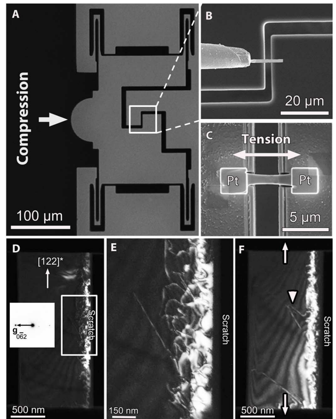
Fig. 2. In situ TEM nanomechanical testing. (A) Optical image of the PTP device used for in situ TEM tensile experiments. The compression of the semi-circular end in (A) induces uniaxial tension in the middle gap shown in (B) and (C). (B and C) Scanning electron microscope (SEM) images showing the transfer of an FIB-prepared olivine sample onto the PTP device and the mounting of the sample in the middle gap using electron beam-deposited platinum (Pt), respectively. (D) WBDF-TEM image of the olivine sample DefOI-4 mounted on the PTP device before deformation. The scratch and the pulling direction are perpendicular to the (112) plane. The sample is oriented in a two-beam condition with the vector g = 062 perpendicular to the pulling direction. (E) Zoom on the damaged layer underneath the polished surface surrounded by the rectangle in (D). Several dislocation loops can be observed. (F) WBDF-TEM image showing the nucleation of a dislocation loop (white arrowhead) in the (110) plane from the damaged layer during in situ TEM straining. The pulling direction is indicated by white arrows in (F).
