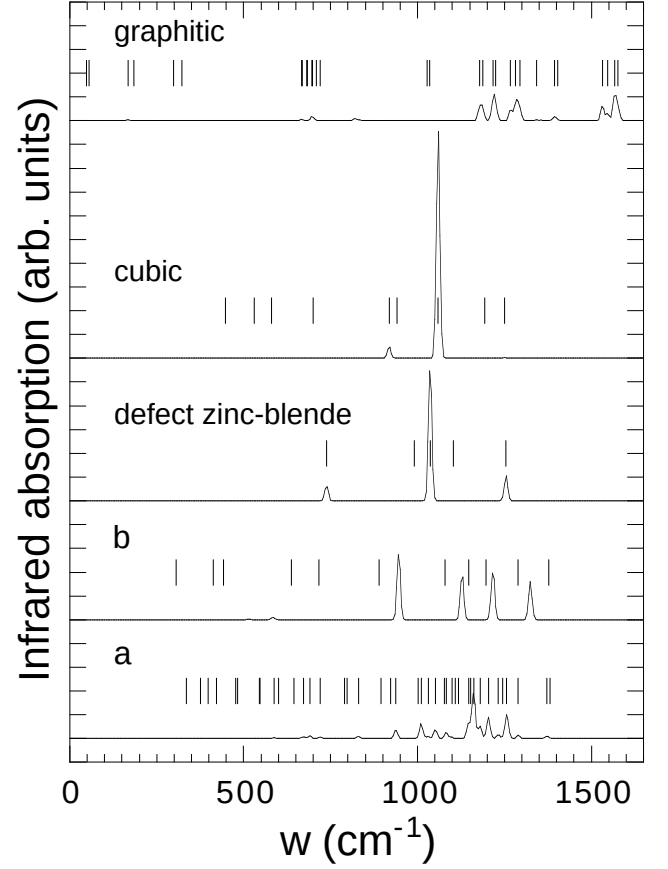
FIG. 1: Infrared absorption spectra for the different C 3 N 4 polymorphs [31]. The Raman frequencies (vertical lines) are also indicated [38].
