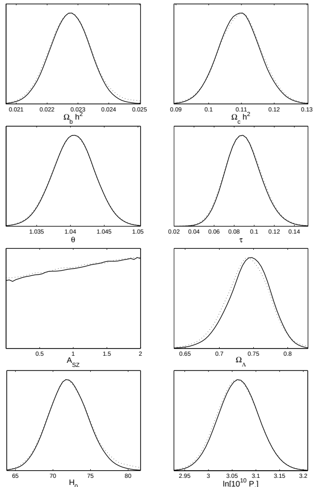
FIG. 1: One dimensional marginalised posterior probability distribution (solid) and mean likelihoods (dotted) for the base and derived cosmological parameters, given the WMAP5 data and the k-inflation power spectra of Eq. (8).
