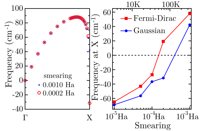
Fig. 6. Effect of the smearing on the Peierls instability for the longitudinal mode of the linear chain at \epsilon = 0.09 . In the left panel, the phonon dispersion curve is illustrated for two different values of the Gaussian smearing: 0.0010 Ha (blue dots) and 0.0002 Ha (red circles). In the right panel, the phonon frequencies at X are reported as functions of the Gaussian (blue curve with circles) or Fermi-Dirac (red curve with squares) smearing. When the smearing is too high, the Peierls instability is hidden.
