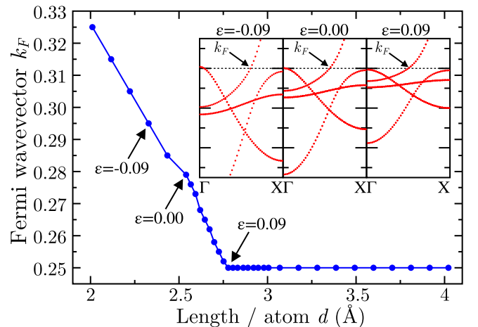
Fig. 7. Evolution of the Fermi wavevector k_F for the linear chain as a function of the length per atom d (expressed in Å). The corresponding electronic bandstructures are illustrated for three different strain values ( \epsilon = -0.09, 0.00 , and 0.09 ).
