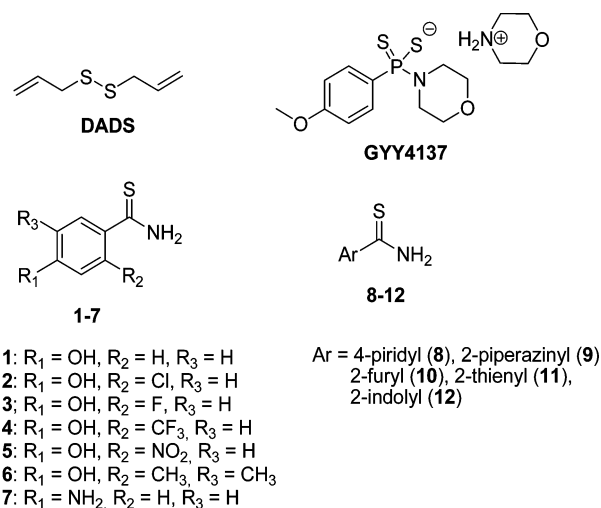
Chart 1. Structures of Known and Newly Synthesized H 2 S-Releasing Agents 1–12
