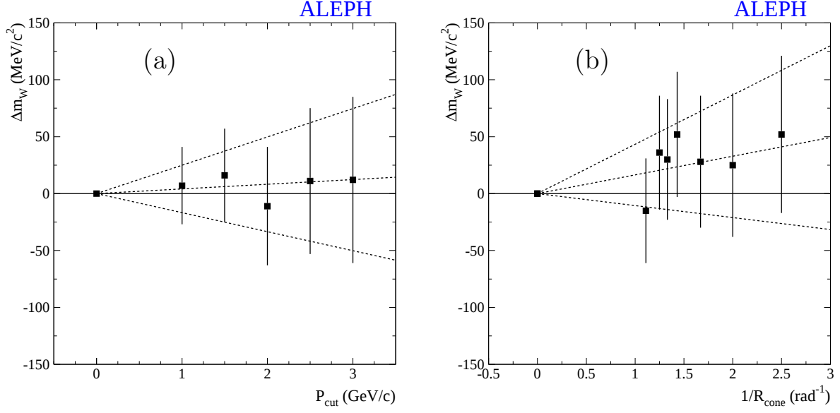
Figure 6: \Delta m_W versus (a) PCUT in GeV/c and (b) inverse CONE radius (R) in rad -1 for data from the e, \mu, \tau\nu q\bar{q} channels combined, fitting with the jets alone in each case
