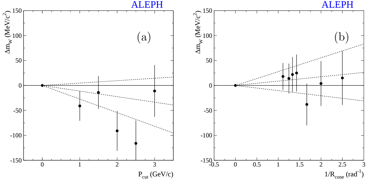
Figure 5: \Delta m_W versus (a) PCUT in \text{GeV}/c and (b) inverse CONE radius ( R ) in \text{rad}^{-1} for qq\bar{q}\bar{q} data. The dashed lines denote the fitted slopes and \pm 1\sigma errors. The correlation with respect to the standard analysis is taken into account in the error on the mass difference for each reconstruction.
