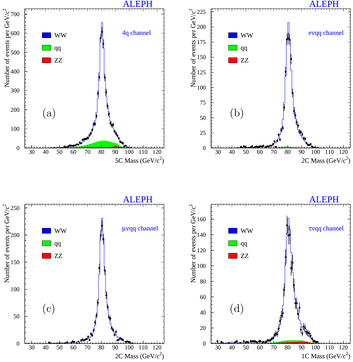
Figure 3: Mass distributions in the: (a) 4q, (b) e\nu q\bar{q} , (c) \mu\nu q\bar{q} and (d) \tau\nu q\bar{q} channels for data (points with error bars), non-WW background (shaded area) and signal+background Monte Carlo with m_W values set to those fitted from each individual channel (solid line histogram). For the 4q channel, the distribution shows the 5C kinematically fitted dijet masses before window cuts are applied. For the \ell\nu q\bar{q} channels, the distributions show the 2C (or 1C) kinematic fits before window cuts.
