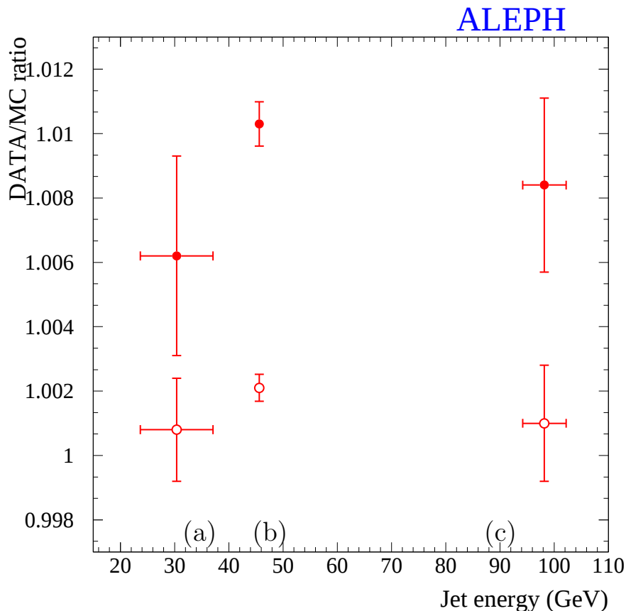
Figure 2: Data/MC ratio of average E_{\text{jet}}/E_{\text{beam}} for E_{\text{jet}} energies of (a) 3-jet events at the Z, (b) di-jet events at the Z and (c) high energy di-jet events. Closed points: |\cos \theta_{\text{jet}}| > 0.7 , open points: |\cos \theta_{\text{jet}}| < 0.7 .
