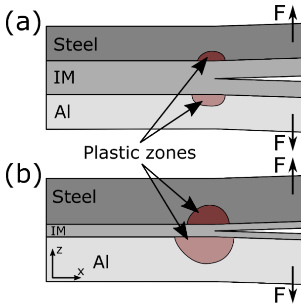
Figure 13: Schematic representation of the increase of plastic zone size in the base materials for welds with a (a) thick and (b) thin IM layer, respectively.
