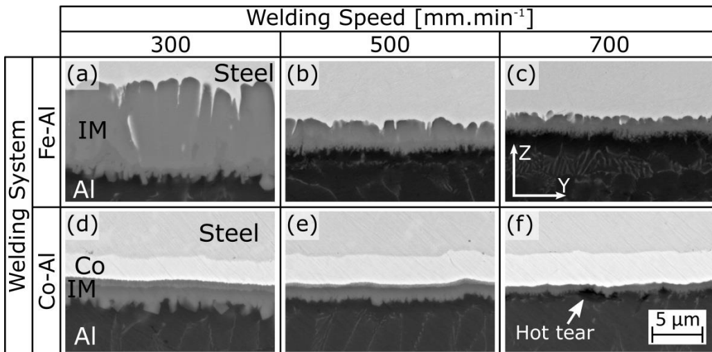
Figure 3: Backscatter SEM micrographs of the intermetallic phases formed at the interface for the Fe-Al and Co-Al welding systems with welding speeds of 300, 500 and 700 \text{ mm}\cdot\text{min}^{-1} .
