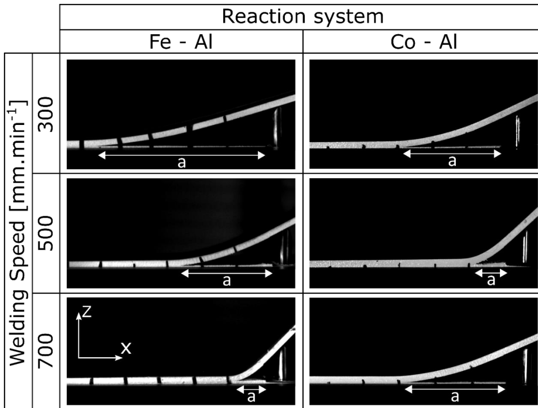
Figure 6: Frames from the video recording of the crack propagation test at a constant rod displacement of 3 mm for the Fe-Al and Co-Al systems at three different welding speeds (300, 500 and 700 \text{mm} \cdot \text{min}^{-1} ). The horizontal black marks on the specimens are spaced of 5 mm starting from the tip of the notch.
