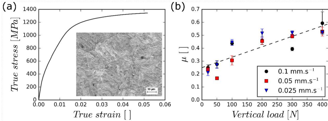
Figure 8: Data used for the calculation of \Gamma . (a) Stress-strain curve of the steel. The insert shows the martensitic microstructure after processing and (b) evolution of the friction coefficient, \mu , as a function of the vertical load for various travel speeds.
