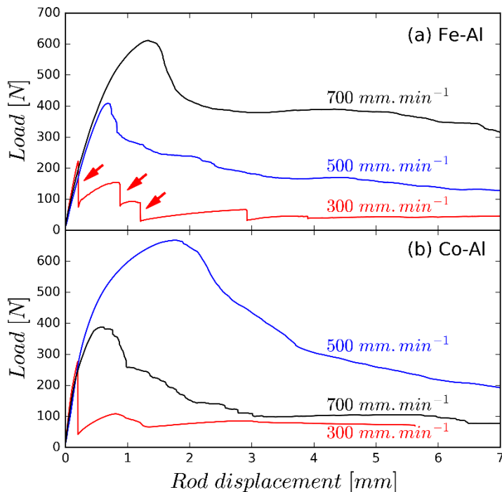
Figure 7: Load-displacement curves of the pushing rod measured during the crack propagation tests for the (a) Fe-Al and (b) Co-Al systems. The red arrows denote a sudden brittle propagation of the crack at 300 \text{mm} \cdot \text{min}^{-1} in the Fe-Al system.
