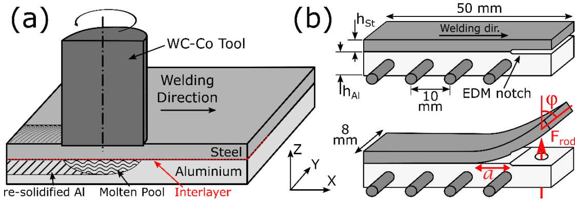
Figure 1: (a) Schematic representation of (a) the FMB process; (b) of the crack propagation tests. F_{rod} represents the load provided by the pushing rod and a represents the crack length measured from the tip of the notch.
