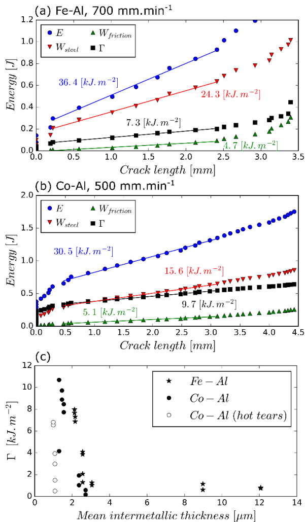
Figure 9: Calculation of the critical energy release rate, \Gamma , on (a) a Fe-Al specimen welded at 700 \text{ mm}\cdot\text{min}^{-1} and (b) a Co-Al specimen welded at 500 \text{ mm}\cdot\text{min}^{-1} . Each point of the curve corresponds to a frame of the video recording. The continuous lines correspond to the linear fit. (c) Calculated critical energy release rates, \Gamma , for the Fe-Al and the Co-Al systems as a function of the mean IM layer thickness. The empty marks denote the presence of hot tears in the specimen.
