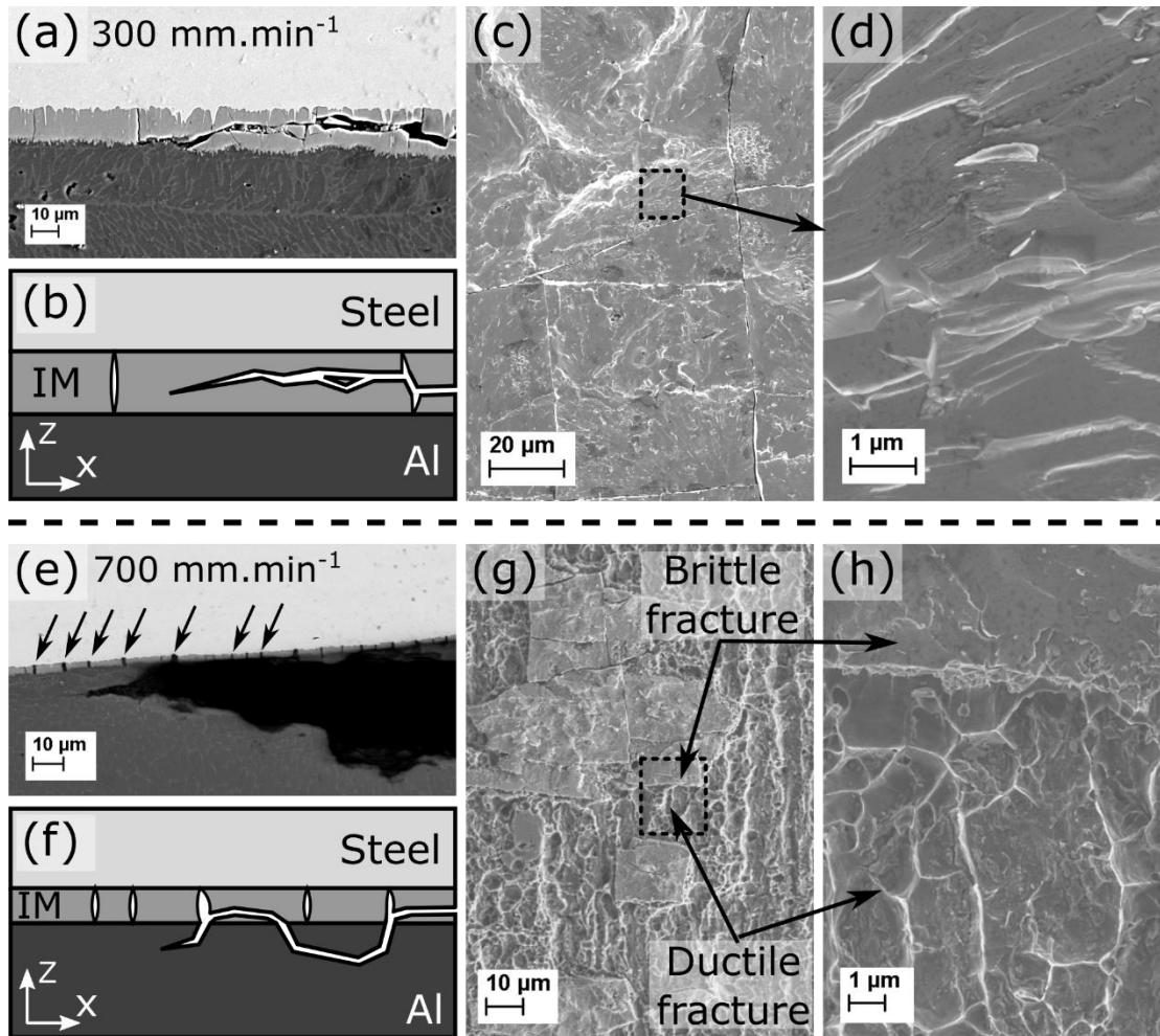
Figure 10: Crack and surface observations for the Fe-Al system corresponding to a weld performed at (a, b, c and d) 300 \text{ mm}\cdot\text{min}^{-1} and (e, f, g and h) 700 \text{ mm}\cdot\text{min}^{-1} . (a and b) Longitudinal cross section and schematic representation of the crack propagation through the IM layer, respectively. (c and d) Surface observations of the fracture revealing a brittle fracture at low and high magnification respectively. (e and f) Longitudinal cross section and schematic representation of the alternating crack propagation through the Al plate and the IM layer, respectively. (g and h) Surface observations of the fracture surface revealing a ductile fracture at low and high magnification respectively.
