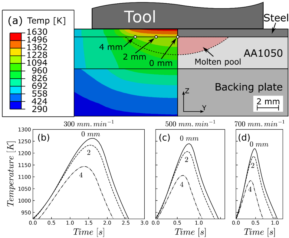
Figure 2: (a) Transversal cross cut view of a simulation of the thermal fields using Abaqus [20] for a weld performed at 700 \text{ mm}\cdot\text{min}^{-1} . (b, c and d) Temperature profiles as a function of time at the steel-aluminium interface from the simulations at 3 different distances from the weld centreline (0 mm, 2 mm and 4 mm) at welding speeds of (b) 300, (c) 500 and (d) 700 \text{ mm}\cdot\text{min}^{-1} . The coordinate system (Y, Z) refers to Fig. 1.
