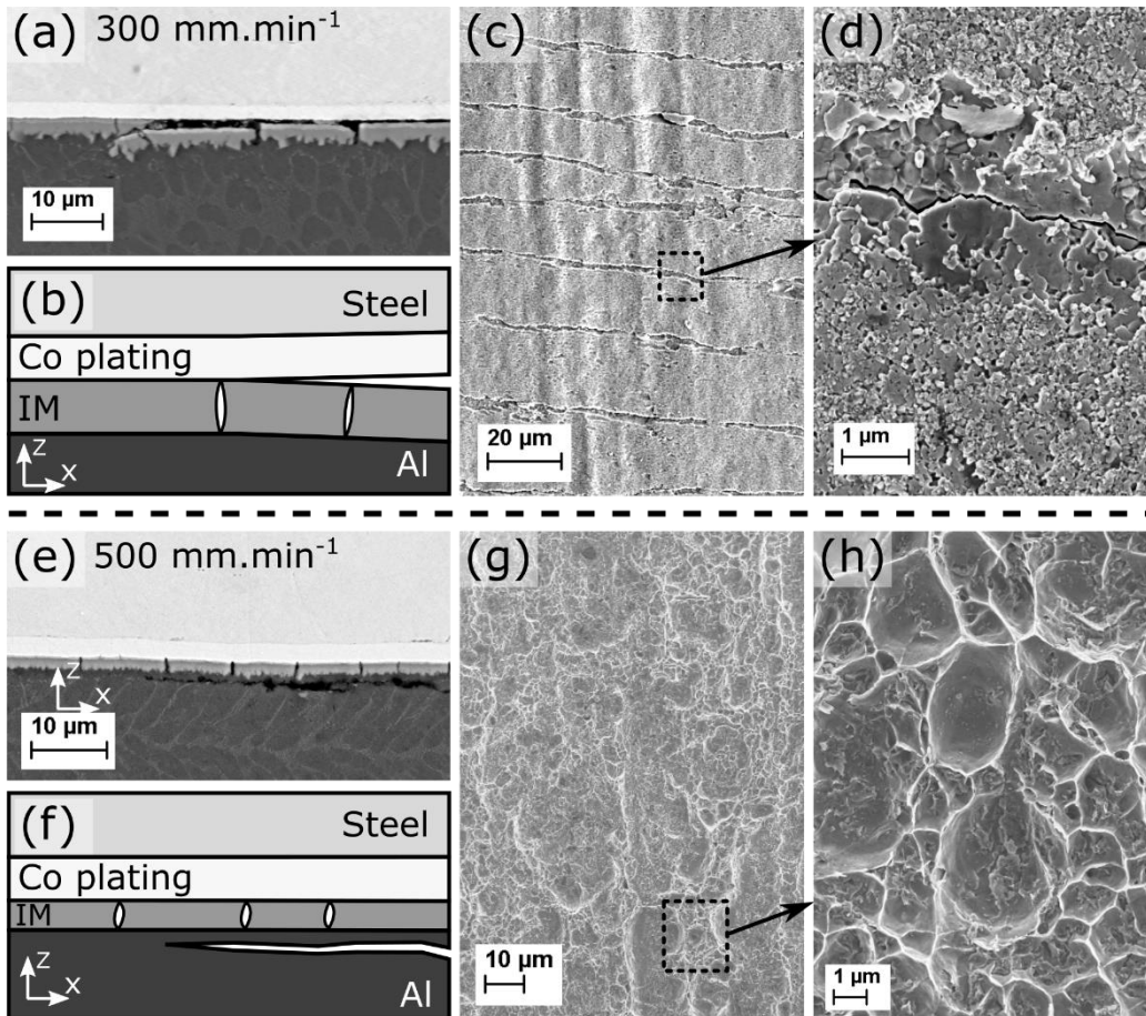
Figure 11: Crack and surface observations for the Co-Al system corresponding to a weld performed at (a, b, c and d) 300 \text{ mm}\cdot\text{min}^{-1} and (e, f, g and h) 500 \text{ mm}\cdot\text{min}^{-1} . (a and b) Longitudinal cross section and schematic representation of the crack propagation through the IM-plating, respectively. (c and d) Surface observations of the fracture revealing the faceted \text{Al}_{13}\text{Co}_4 grains on the Al side of the fracture. (e and f) Longitudinal cross section and schematic representation of the crack propagation through the Al, respectively. (g and h) Surface observations of the fracture surface revealing a ductile fracture characterised by dimples at low and high magnification respectively.
