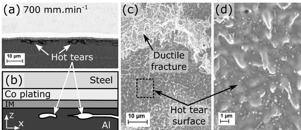
Figure 12: Crack and surface observations for a weld with a Co interlayer at 700 \text{ mm}\cdot\text{min}^{-1} . (a and b) Longitudinal cross section and schematic representation, respectively, of the crack propagation through the Al and the hot tear defects. (c) Surface observation of the fracture surface revealing a combination of hot tears and ductile fracture surfaces. (d) Observation at high magnification of the surface of a hot tear showing a solidification structure.
