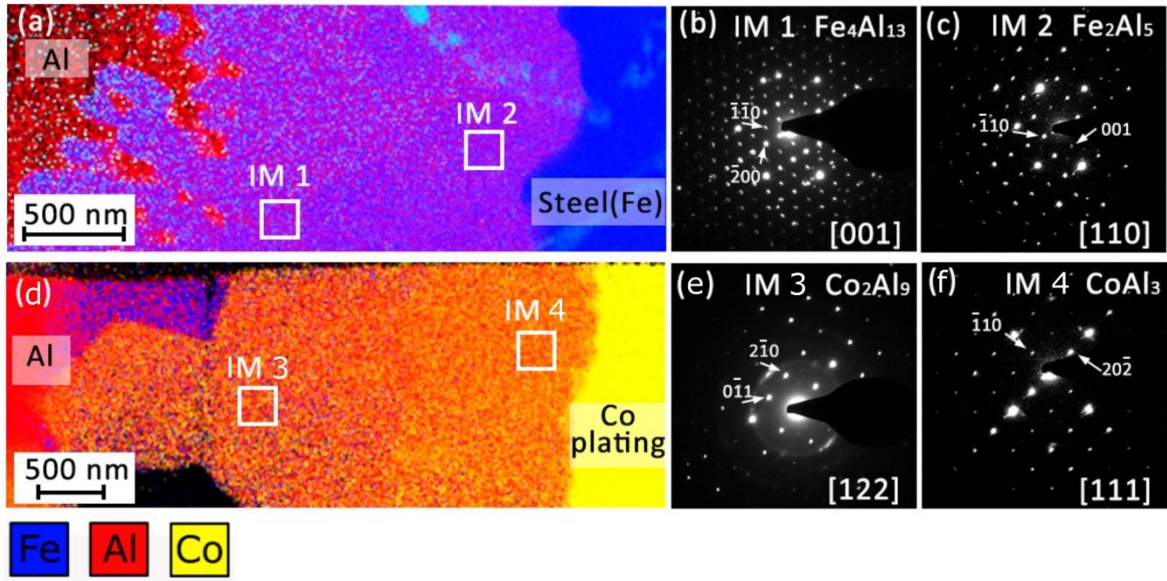
Figure 4: (a and d) EDX elemental maps acquired on FIB samples of the Fe-Al and Co-Al systems, respectively. (b, c, e and f) are SAED patterns obtained on IM1, IM2, IM3 and IM4, respectively, with indicated zone axis corresponding to the identified phase.
