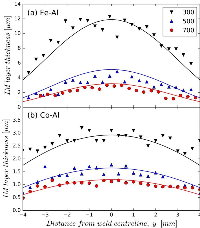
Figure 5: Thickness of the IM layer in the (Y, Z) plane (defined in Fig. 1). The points represent the measured thickness from the SEM images. The continuous lines are drawn using Eqs. 2 and 3 with the fitted parameters given in Table 7 and the temperature field from the FE simulations. Results are provided for the welding systems, (a) Fe-Al, and (b) Co-Al, at three welding speeds (300, 500 and 700 \text{mm}\cdot\text{min}^{-1} ).
