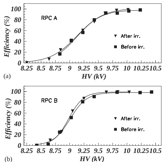
Fig. 2. Efficiency of RPC A in (a) and RPC B in (b) as a function of HV before and after the irradiation.
