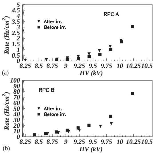
Fig. 3. Noise rate of RPC A in (a) and RPC B in (b) as a function of HV before and after the irradiation.
