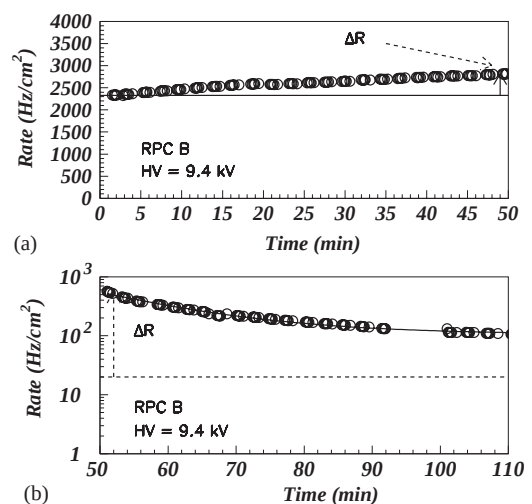
Fig. 1. Counting rate of RPC B (at constant HV) as a function of time during the first irradiation cycle.
