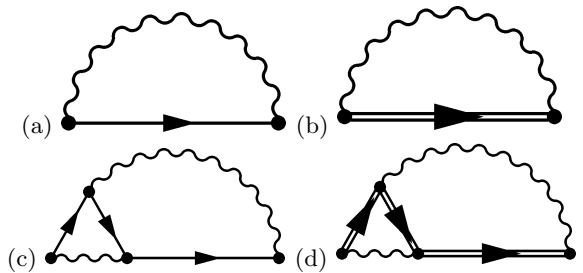
FIG. 1: Different levels of approximation for the one-particle self-energy \Sigma = \Sigma^{(1)} + \Sigma^{(2)} within the plasmon model. First order diagrams: (a) \Sigma^{(1)} = G_0 W_p with G_0 being the bare core-electron Green's function; (b) \Sigma^{(1)} = G W_p for self-consistent calculations. Second order diagrams with vertex corrections (c) \Sigma^{(2)} = G\Gamma_{(1)}^{GW}W_p for non self-consistent calculations; (d) \Sigma^{(2)} = G\Gamma_{(1)}^{SC}W_p for the full self-consistent calculations (see Appendix C 2).
