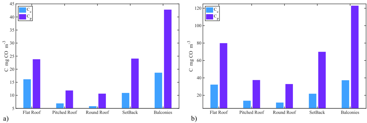
Fig. 10. Street canyon pollutant exchange: the blue colour bars display the C_c results (the PC contained between HP_1 and HP_2 ) while the purple colour displays the C_p results (the PC contained below HP_2 ) a) shows the results obtained for a ventilation efficiency of \eta_p = \eta_c = 1 , while b) shows the results obtained for a ventilation efficiency of \eta_p = \eta_c = 0.5 . (For interpretation of the references to colour in this figure legend, the reader is referred to the web version of this article.)
