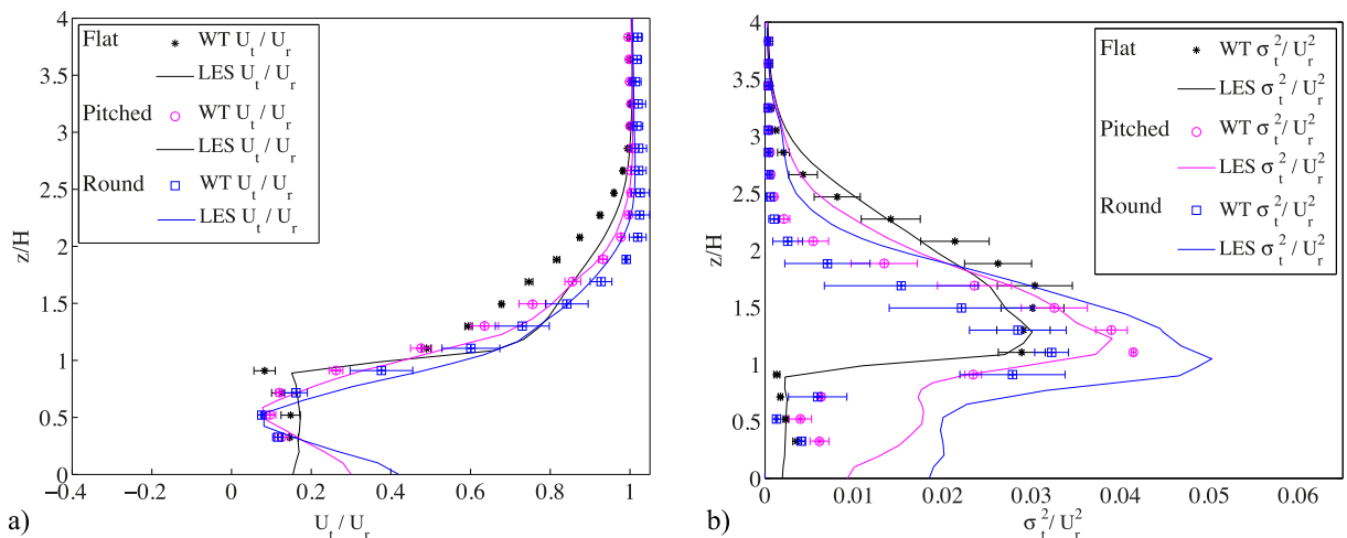
Fig. 4. Wind tunnel and LES result (with imposed Inlet #1 inflow conditions) comparison for canyon #6 until 4H . All values are normalized by the reference velocity U_r , which has been taken at 2.5H upstream. The left panel depicts the wind tunnel and LES wind speed, U_t , for the Flat roof, Pitched roof, and Round roof. U_t is the magnitude of the velocity vector, mainly composed of the streamwise and vertical components. The right panel depicts the corresponding wind tunnel and LES total variances \sigma_t^2 . For more details refer to Llaguno-Munitxa et al. (2017).
