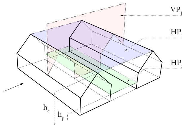
Fig. 5. Air Exchange HP_1 and HP_2 and section plane VP_1 locations. The figure illustrates a limited section of the canyons; and VP_1 is in the middle of the domain span, halfway between the side walls.
