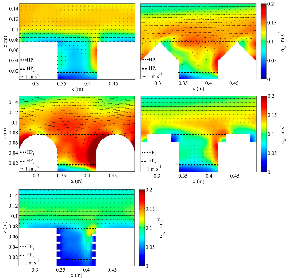
Fig. 6. LES results for air flow and vertical turbulence intensity for the 5 different building geometries. The time-averaged velocity is displayed with the vector plot, and \sigma_w with pseudocolor plots. The thick dashed lines denote the locations of the exchange planes considered.
