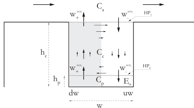
Fig. 9. Street canyon pollutant exchange diagram.
