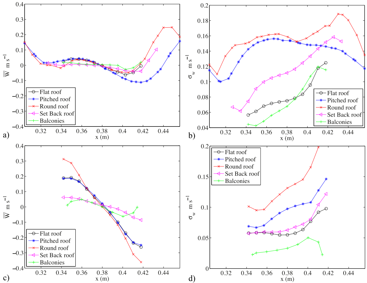
Fig. 7. LES results for spatially-averaged (along the street canyon longitudinal axis, y-direction) exchange planes HP_1 and HP_2 : a) the mean vertical velocity \bar{w} for HP_1 ; b) \sigma_w for HP_1 ; c) the mean vertical velocity \bar{w} for HP_2 ; and d) \sigma_w for HP_2 . Note that the rakes displayed in the figure, show the data computed for the ACH planes HP_1 and HP_2 , which only cover the central area of the canyon, thus the portions adjacent to the walls have not been included (which explains why the mean velocity averages over x would not be exactly 0 for all cases).
