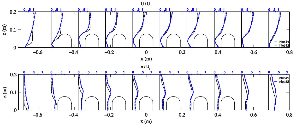
Fig. 3. The top figure displays the normalized mean velocity magnitude for the round roof geometry for the central axis of all 6 canyons (flow is from left to right). The bottom figure displays the total root mean square (rms) velocity \sigma_r for the central axis of all 6 canyons. Two inlet conditions are displayed (inlet #1 and inlet #2) as will be described in Section 3.
