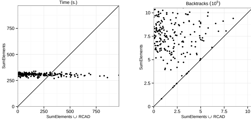
Fig. 7 Comparison of SumElements and SumElements \cup RCAD on large instances.
