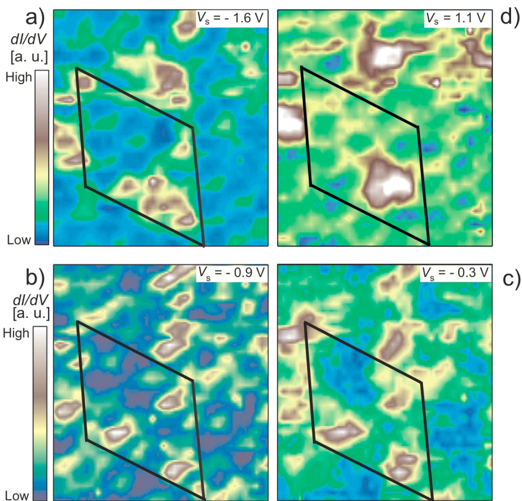
SI-3 : Figure 3. Spectroscopic imaging at 77 K of the Si(111)-7x7 surface with adsorbed MSP assemblies – 5 \times 4 \text{ nm}^2 , for V_s = -1.6, -0.9, -0.3 and 1.1 \text{ V} . Maps (a-c) show the spatial extent of the filled states, with different contributions from the occupied Si rest atom and adatom states at various tunneling voltages. The map at V_s = 1.1 \text{ V} reveals the spreading of the empty states in the decorated faulted half cell over the Si rest atoms and center adatoms due to the presence of the three pyridinium rings.
