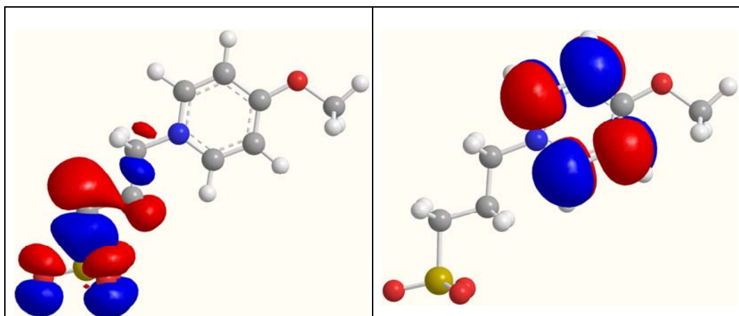
SI-1 : Figure 1. Electronic density in HOMO (Left) and LUMO (right) of the MSP molecule calculated in the vacuum (Blue: positive, red: negative).
