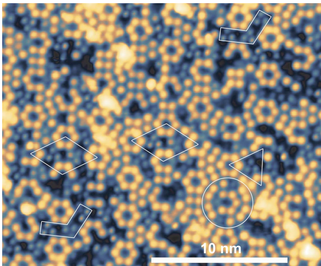
SI-2 : Figure 2. STM image at 77 K of the decorated Si(111)-7x7 surface with MSP molecules – 20 \times 24 \text{ nm}^2 , I = 100 \text{ pA} , V_s = 1.9 \text{ V} .
