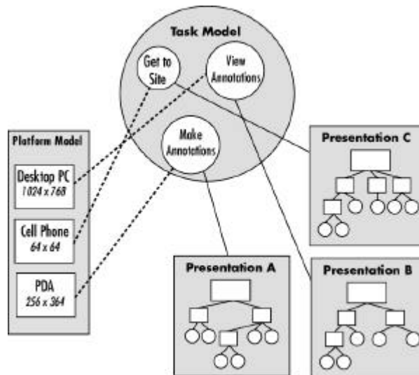
Figure 7. Platform elements are mapped onto high-level task elements that are especially likely to be performed. In turn, the task elements are mapped onto presentation models that are optimized for the performance of a specific task.
