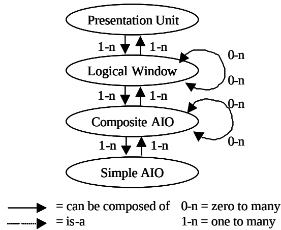
Figure 6. Hierarchy of presentation concepts.
