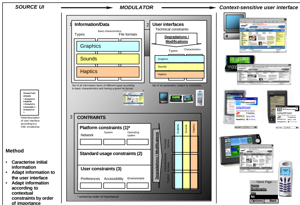
Figure 3. Software architecture of the modulator
