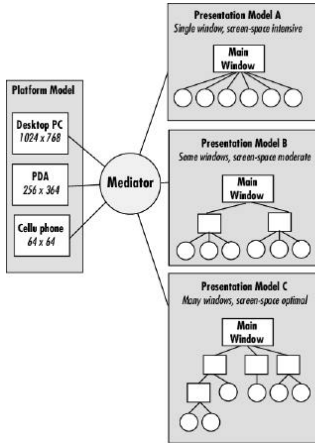
Figure 5: A modulator agent dynamically selects the appropriate presentation model for each device.
