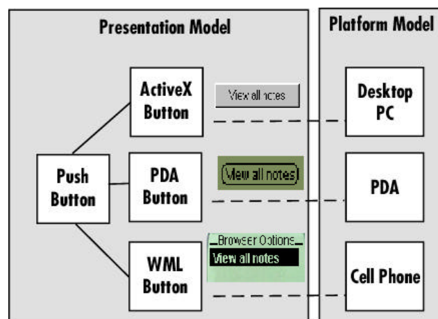
Figure 4. Concrete Interaction Objects are subclassed from an Abstract Interaction Object, and are then mapped on to specific platforms.
