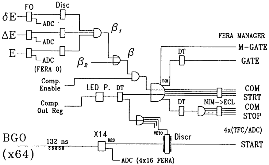
Fig. 5. Schematic diagram of the polarimeter electronics.
