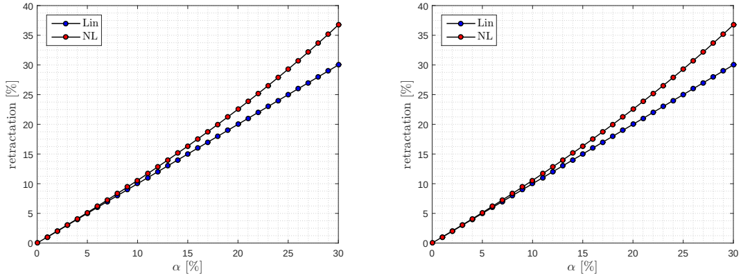
Figure 3.16 – Radius evolution with respect to hydric parameter \alpha_{\mathcal{R}} for the linear and nonlinear formulations for 2D and 3D.
