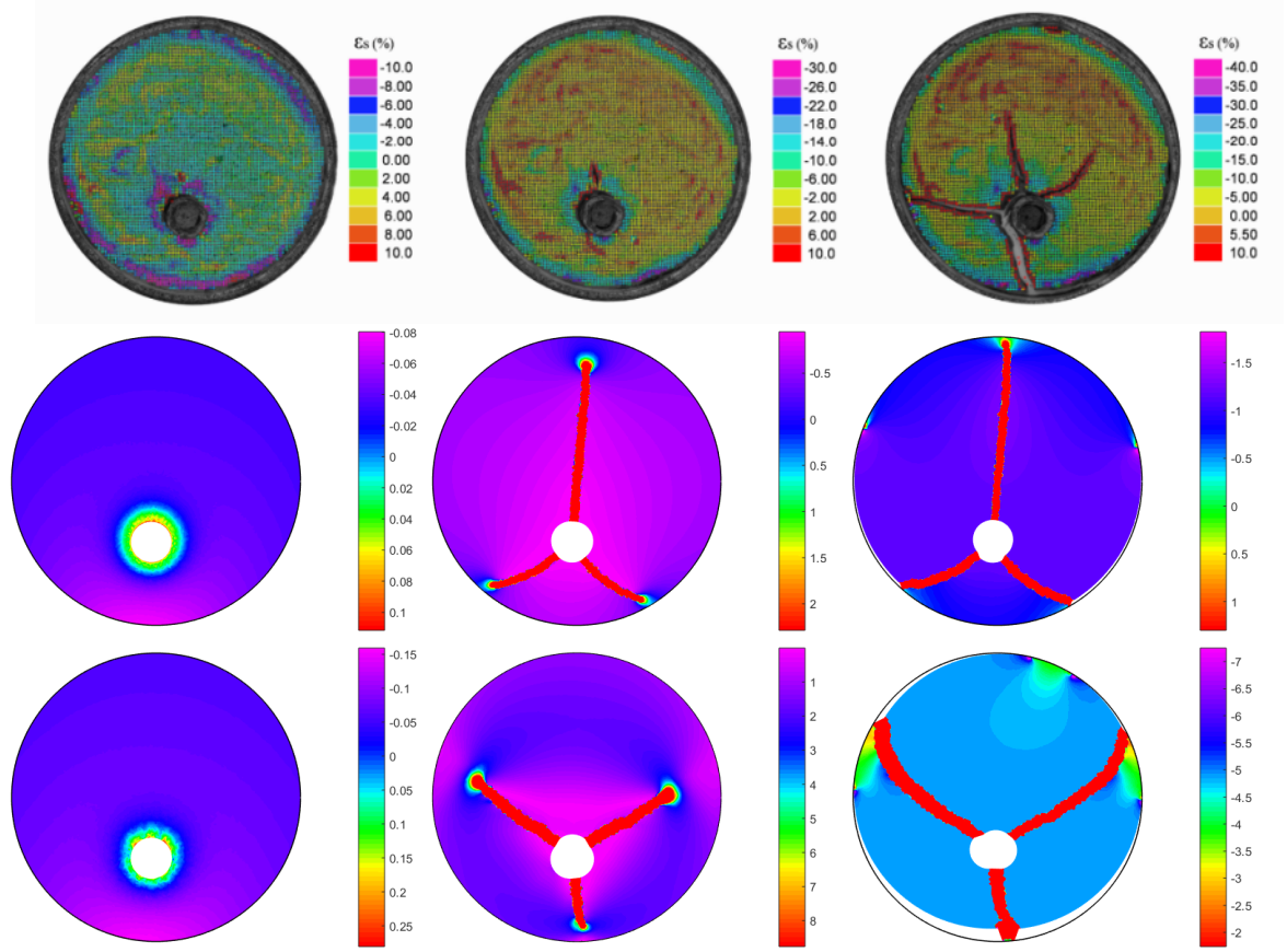
Figure 5.8 – Spherical strain map in S_1 : experimental results (top), numerical results in 2D (middle), and numerical results in 3D (bottom) at times t_1 , t_2 , and t_3 (from left to right).
