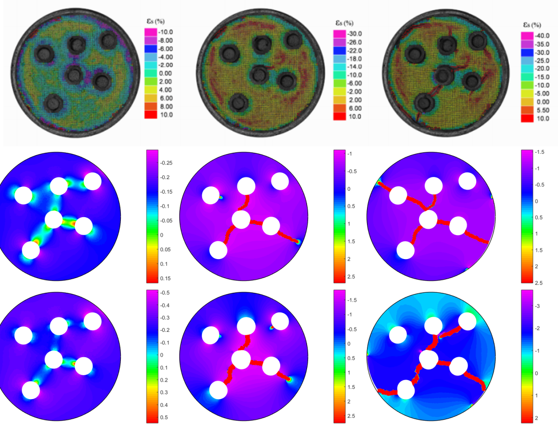
Figure 5.10 – Spherical strain map in S_6 : experimental results (top), numerical results in 2D (middle), and numerical results in 3D (bottom) at times t_1 , t_2 , and t_3 (from left to right).
