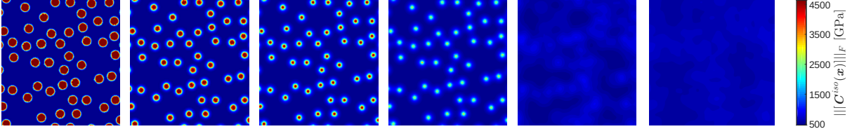
Figure 2.7 – One realization of the random field \{||[\tilde{\mathbf{C}}_{KUBC}^{iso}(\mathbf{x})]||_F, \mathbf{x} \in \Omega\} for \tilde{R}/R \in \{0.2, 0.6, 0.8, 1, 2, 4\} (from left to right).
