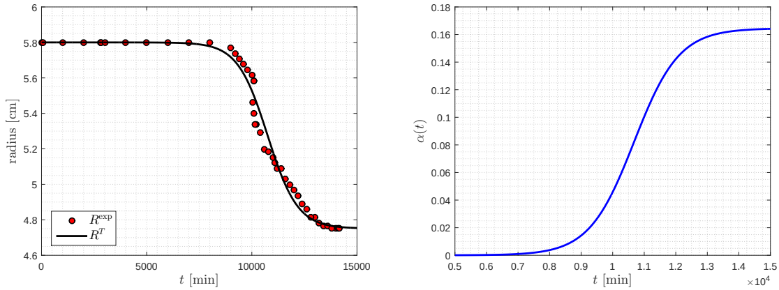
Figure 5.2 – (Left) Identified R^T function, (right) the identified shrinkage parameter \alpha_R .
