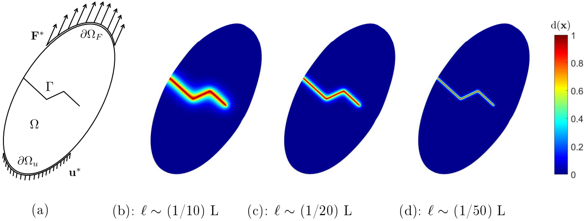
Figure 1.14 – (a) sharp description of a cracked solid; (b), (c), (d): smeared description within the phase field framework (damage profiles d \in (0, 1) for different regularization lengths \ell ).
