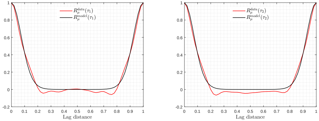
Figure 2.19 – Normalized correlation function of the shear modulus random field along \mathbf{e}^{(1)} (left) and \mathbf{e}^{(2)} (right), estimated from the multiscale data (red line) and the calibrated stochastic model (black line).
