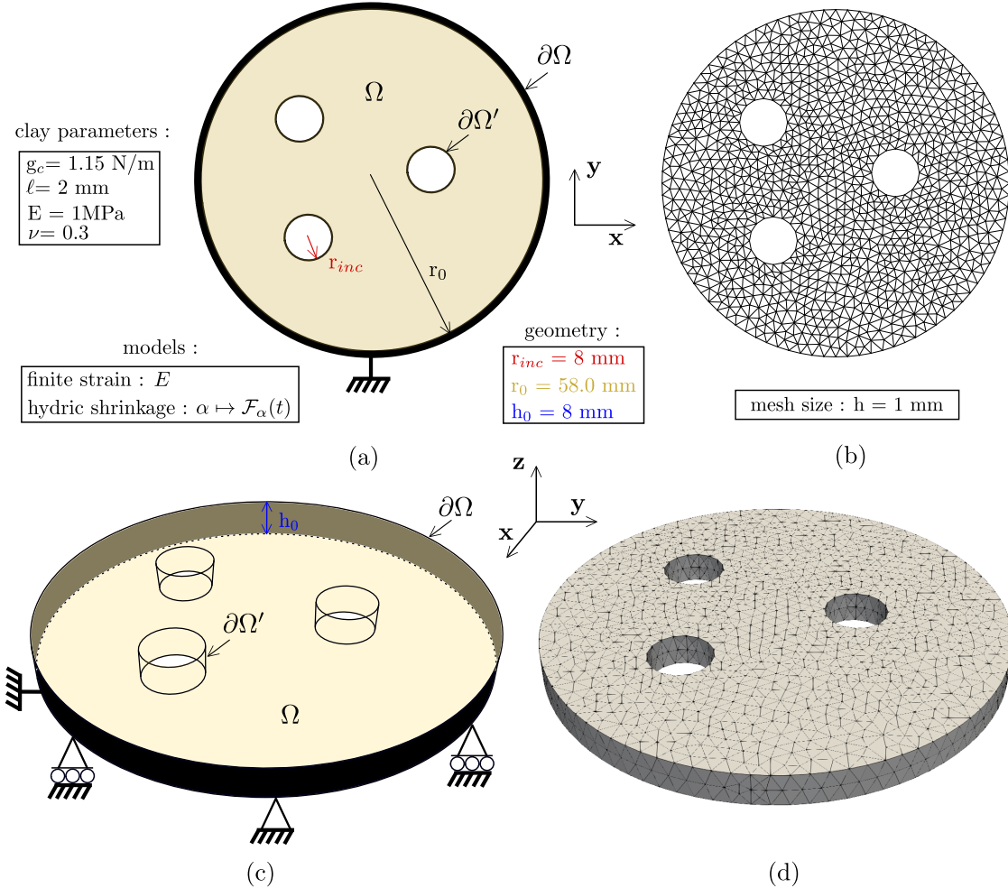
Figure 5.1 – Problem definition for a specific configuration: (a) geometry and boundary conditions for the 2D model; (b) 2D mesh; (c) geometry and boundary conditions for the 3D model; (d) 3D mesh.
