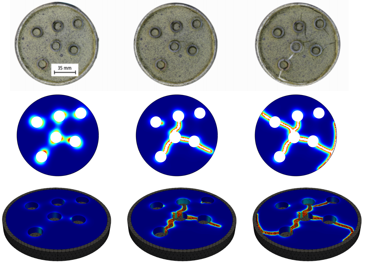
Figure 5.6 – Crack pattern S_6 : experimental results (top), numerical results in 2D (middle), and numerical results in 3D (bottom) at times t_1 , t_2 , and t_3 (from left to right).
