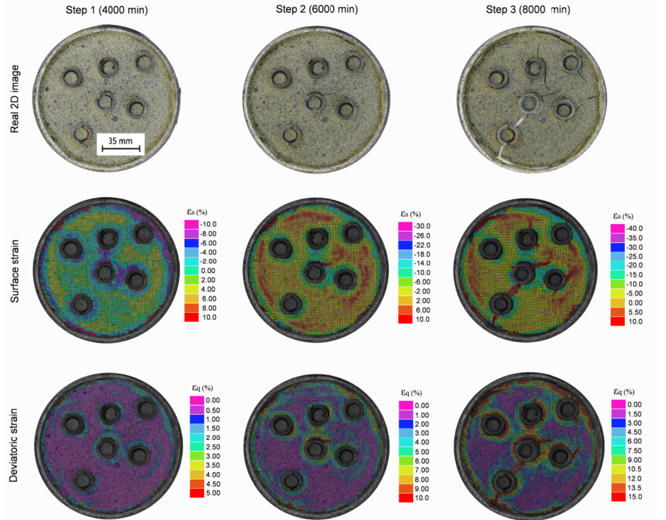
Figure 4.10 – S_6 test with shrinkage, spherical and deviatoric strain for t = 4000, 6000 , and 8000 min.
