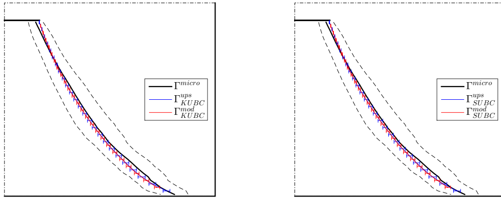
Figure 2.20 – Comparison of crack paths obtained with the microscopic description (black dashed/solid lines), the mesoscopic formulation where the elasticity is obtained from microstructural samples (blue lines), and the mesoscopic formulation involving the stochastic model for elasticity tensors (red lines). Left panel: case of KUBC. Right panel: case of SUBC.
