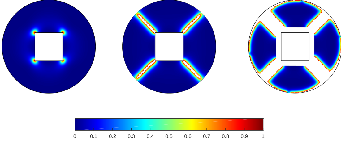
Figure 3.20 – Different shrinkage states \alpha_{\mathcal{R}} = 0.01\% - 1\% - 10\% .
