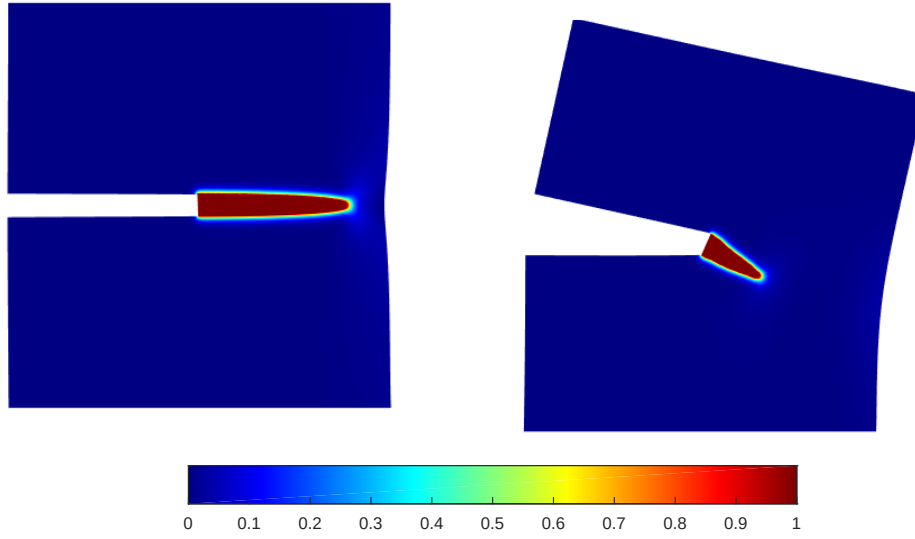
Figure 3.4 – Crack path illustration for: M_I (left) and M_{II} (right) tests.
