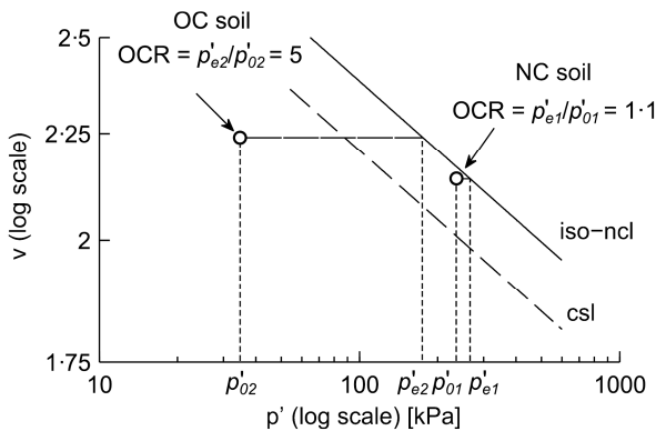
Figure 2. Considered initial states in the compression plane.
