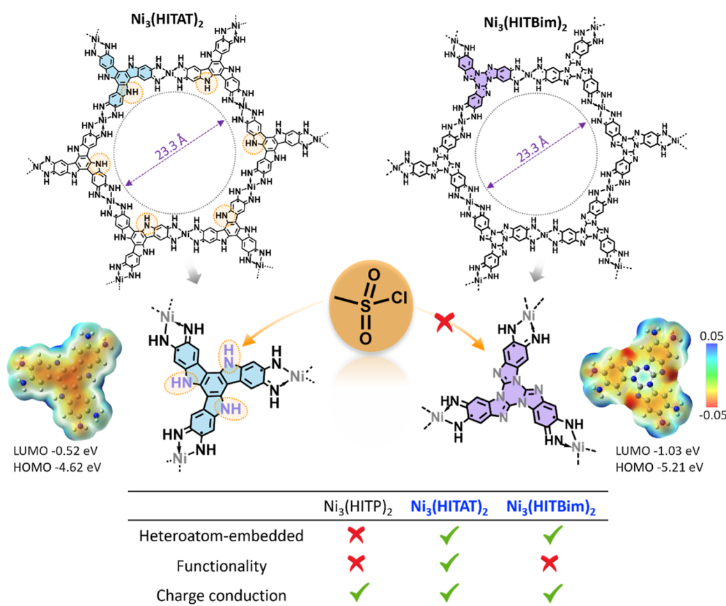
Figure 1. Molecular design of Ni 3 (HITAT) 2 and Ni 3 (HITBim) 2 MOFs (top). Molecular electrostatic potential maps of the corresponding ligands HATAT and HATBim and the computed HOMO and LUMO levels highlight the electron-deficient character of the HATBim as compared to HATAT. (bottom table) Comparative analysis of key properties between archetypal Ni 3 (HITP) 2 and the Ni 3 (HITAT) 2 as well as Ni 3 (HITBim) 2 MOFs presented in this work.
