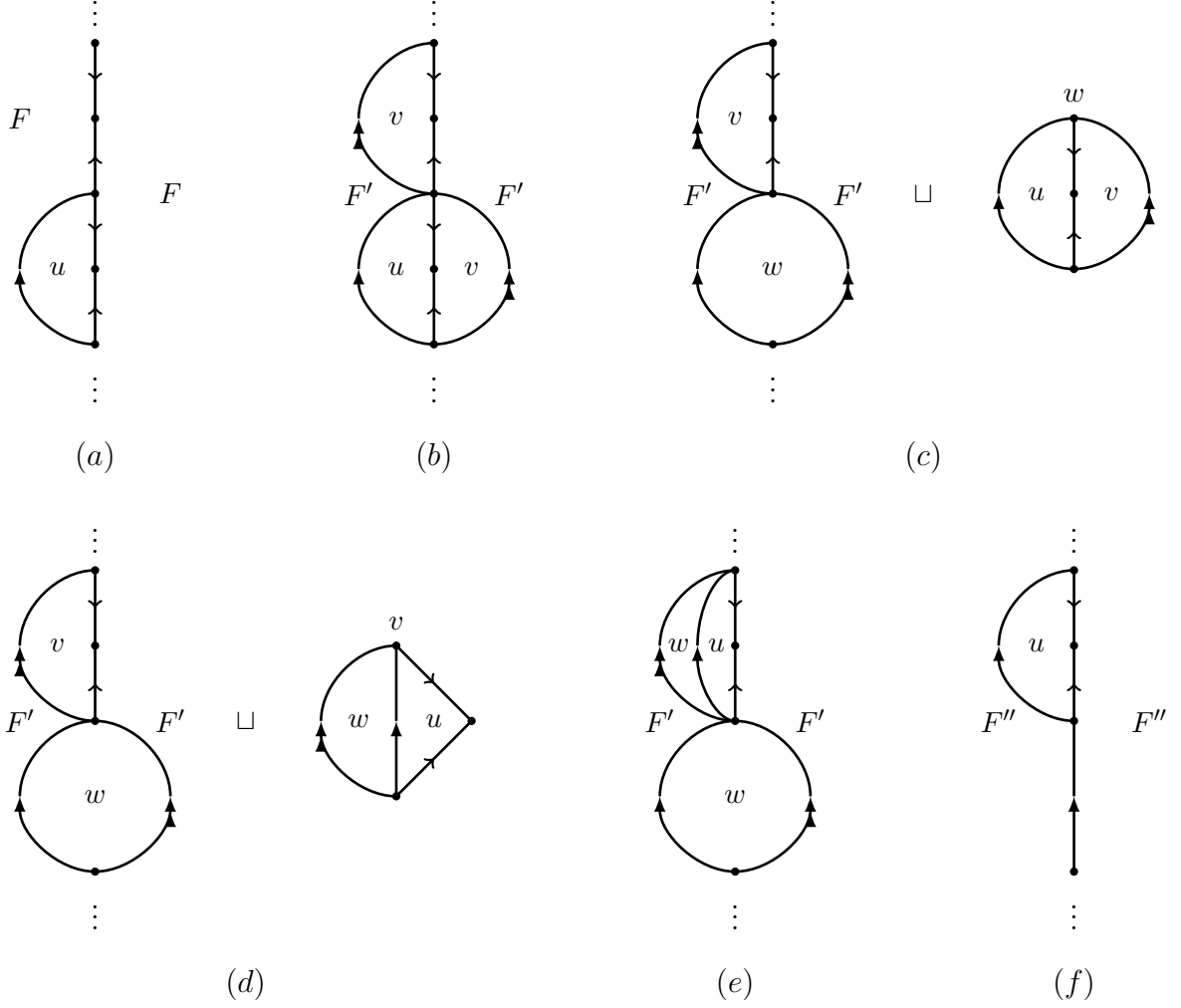
FIGURE 10. The bigon trick
