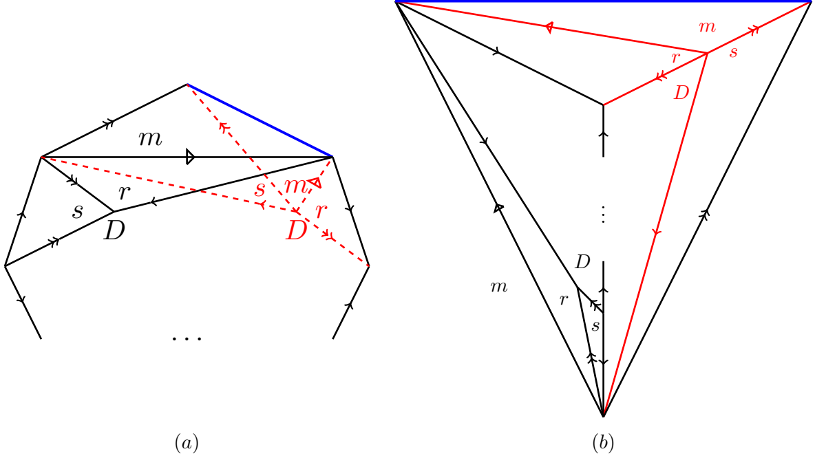
FIGURE 9. A cellular decomposition of (S^3, K_n) as a polyhedron glued to itself
