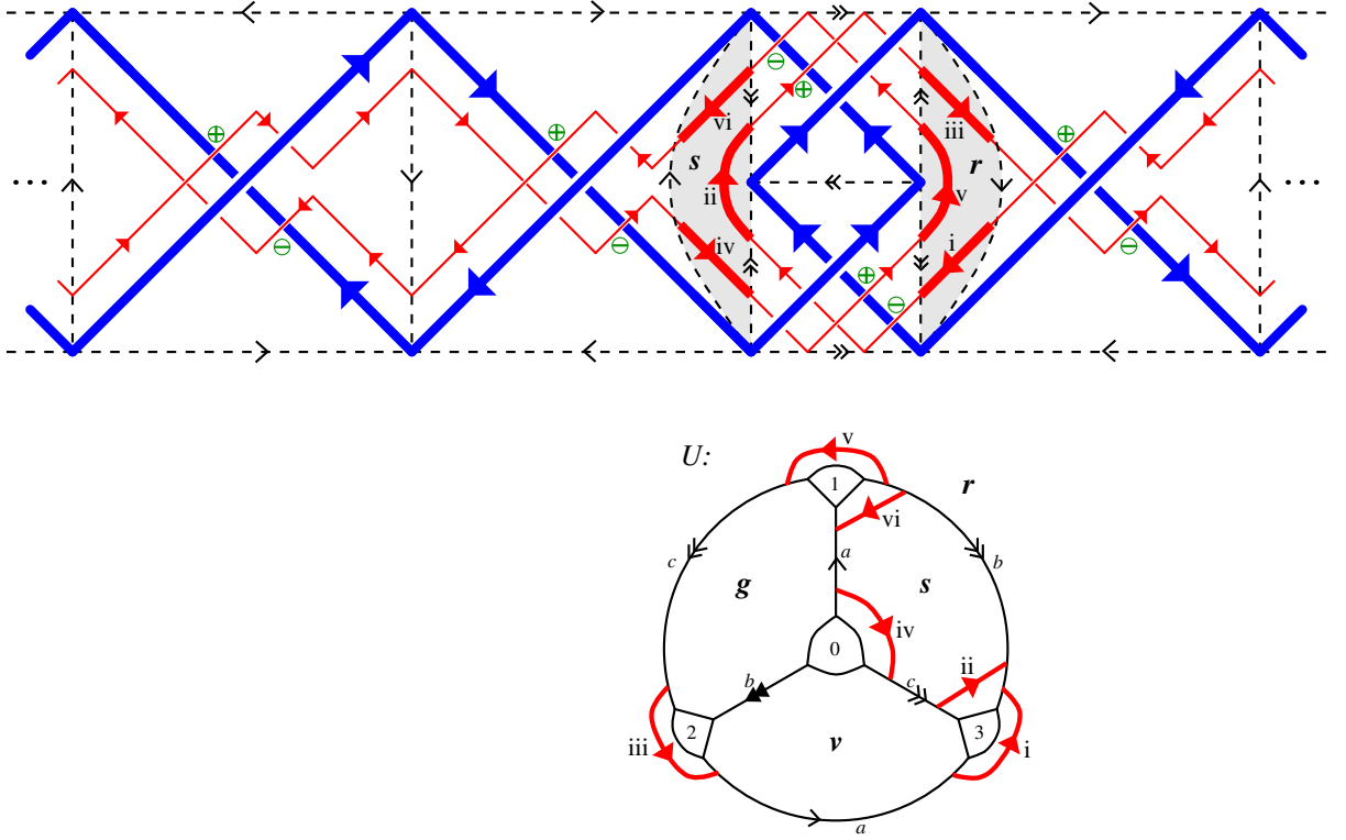
FIGURE 16. A preferred longitude l_{X_n}^0 = (i) \cup \dots \cup (vi) (in red) for the odd twist knot K_n , seen in S^3 \setminus K_n (top) and on the truncated tetrahedron U (bottom).
