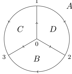
FIGURE 1. The positive tetrahedron T
