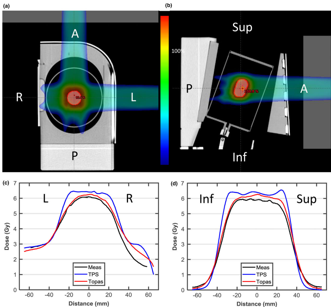
FIG. 10. (a, b) Axial and sagittal view of the proton lung phantom with gantry angle orientation indicated. (c, d) Dose profile through the center of the planning target volume (PTV) in the left-right and inferior-superior directions. Film measurements are shown in black, the analytic pencil beam algorithm in blue, TOPAS.
