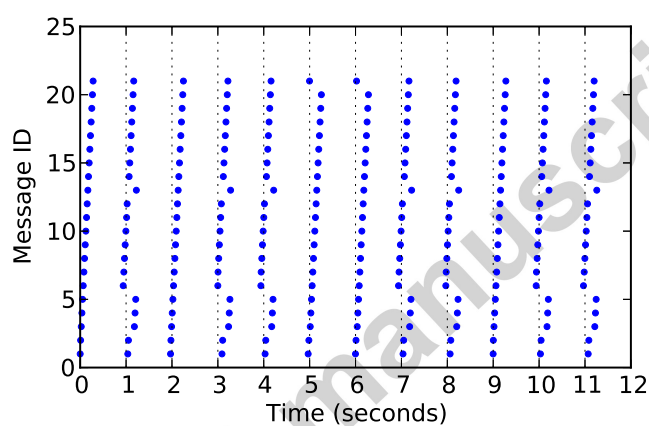
(b) Flow with unordered requests.
