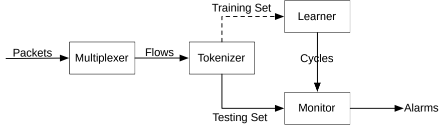
Figure 1: PeriodAnalyser evaluation approach.
