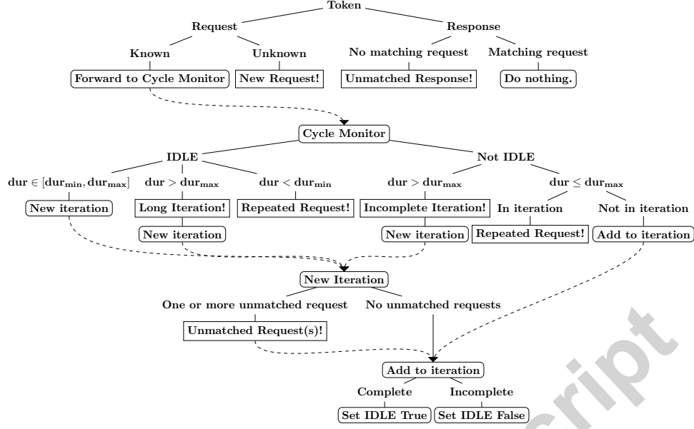
Figure 2: Decision graph used by the Monitor module.
