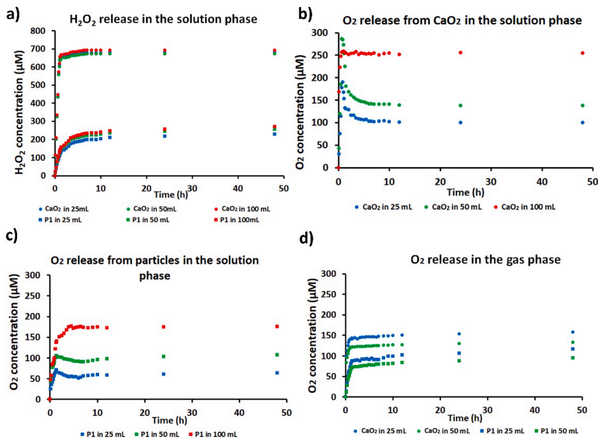
Fig. 6. (a) H_2O_2 release from CaO_2 and P1 particles in 25, 50, and 100 mL of the solution phase, (b) O_2 release from CaO_2 in 25, 50, and 100 mL of the solution phase, (c) O_2 release from P1 particles in 25, 50, and 100 mL of the solution phase, and (d) O_2 release from CaO_2 and P1 in the gas phase when the volume of the solution phase is 25 and 50 mL.
