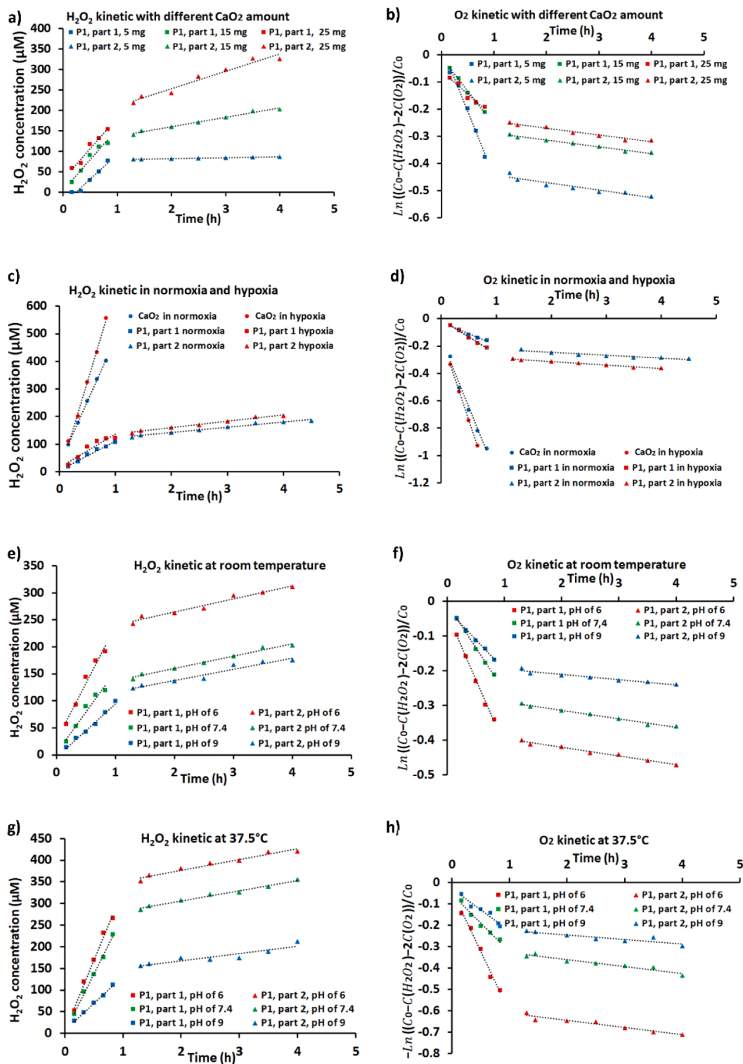
Fig. 9. The kinetics of \text{O}_2 and \text{H}_2\text{O}_2 (a and b) of 5, 15, 25 mg of \text{CaO}_2 and a certain amount of P1 particles containing 5, 15, 25 mg of \text{CaO}_2 , (c and d) of \text{CaO}_2 and P1 particles in hypoxia and normoxia (e and f), of P1 particles in hypoxia and different pHs at room temperature, and (g and h) of P1 particles in hypoxia and different pHs at 37^\circ\text{C} .
