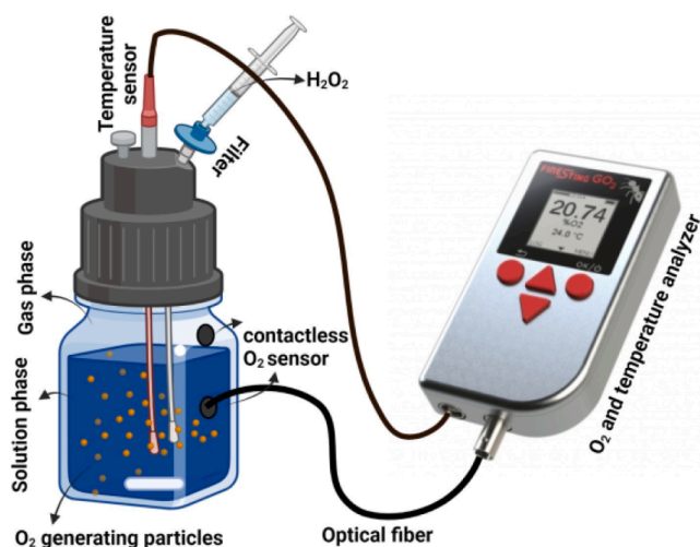
Fig. 1. Experimental procedure to determine the amount of O 2 in the gas and solution phases and of H 2 O 2 in the solution phase.
