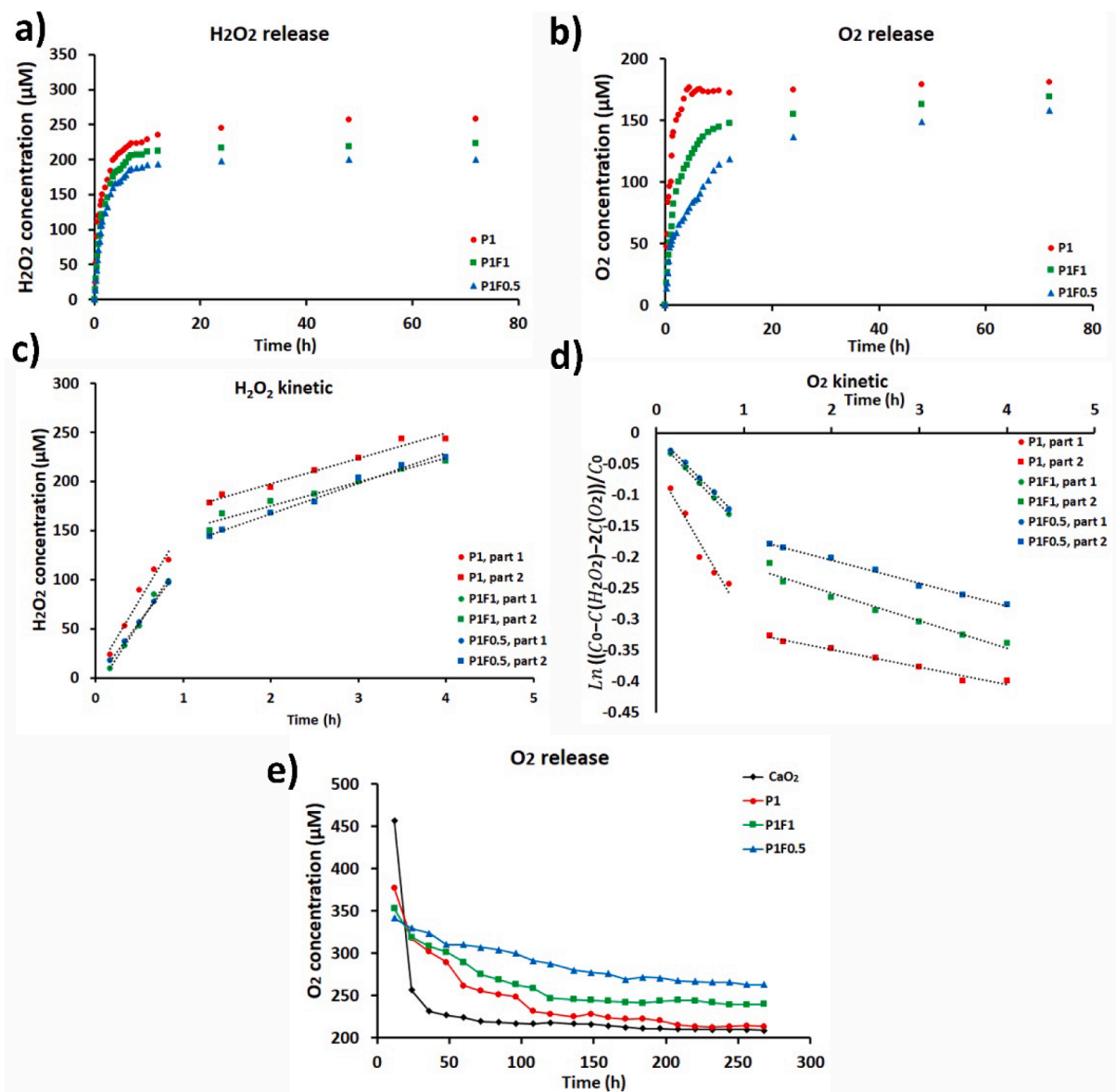
Fig. 10. (a and b) H 2 O 2 and O 2 release from P1, P1F0.5, and P1F1, (c and d) the kinetics of H 2 O 2 and O 2 from P1, P1F0.5, and P1F1, and (e) O 2 preserving of CaO 2 , P1, P1F0.5, and P1F1 at pH of 7.4 and the room temperature in 100 mL of the release media with normoxia condition.
