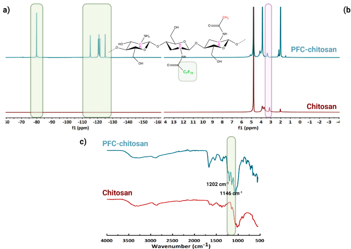
Fig. 3. (a) ^{19}\text{F} NMR, (b) ^1\text{H} NMR and (c) FTIR of the chitosan and the PFC-chitosan film.
