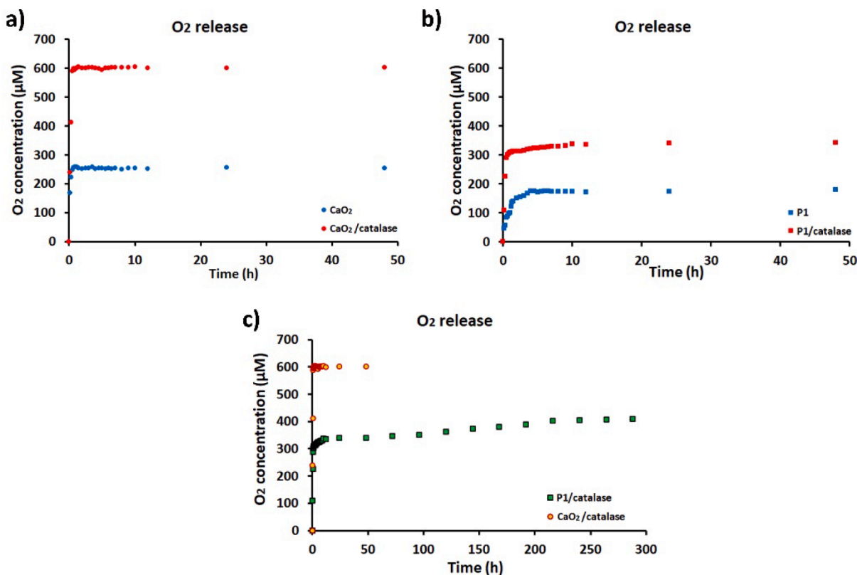
Fig. 8. (a) \text{O}_2 release from 15 mg of \text{CaO}_2 with and without catalase in 100 mL of DI water, (b) \text{O}_2 release from a certain amount of P1 particles containing 15 mg of \text{CaO}_2 with and without catalase in 100 mL of DI water, (c) \text{O}_2 release from 15 mg of \text{CaO}_2 and a certain amount of P1 particles containing 15 mg of \text{CaO}_2 with catalase until 288 h.
