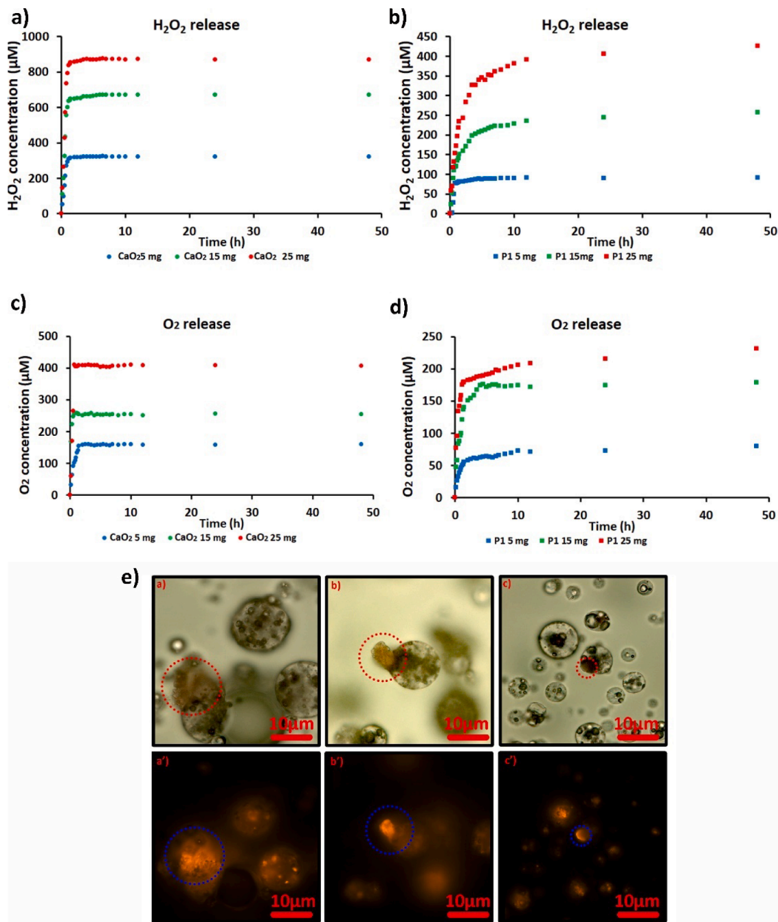
Fig. 7. (a) H 2 O 2 release from 5, 15, and 25 mg of CaO 2 , (b) H 2 O 2 release from a certain amount of P1 particles containing 5, 15, 25 mg CaO 2 , (c) O 2 release from 5, 15, and 25 mg of CaO 2 , (d) O 2 release from a certain amount of P1 particles containing 5, 15, 25 mg CaO 2 , and (e) the microscopic (a-c) and fluorescent images (a'-c') of the loaded CaO 2 in the outer layer of the PCL particles.
