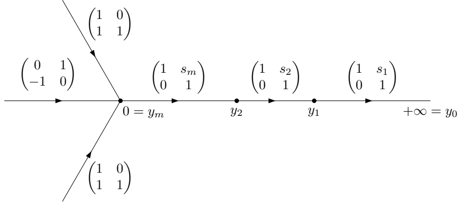
Figure 1: Jump contours for the model RH problem for \Psi with m = 3 .
