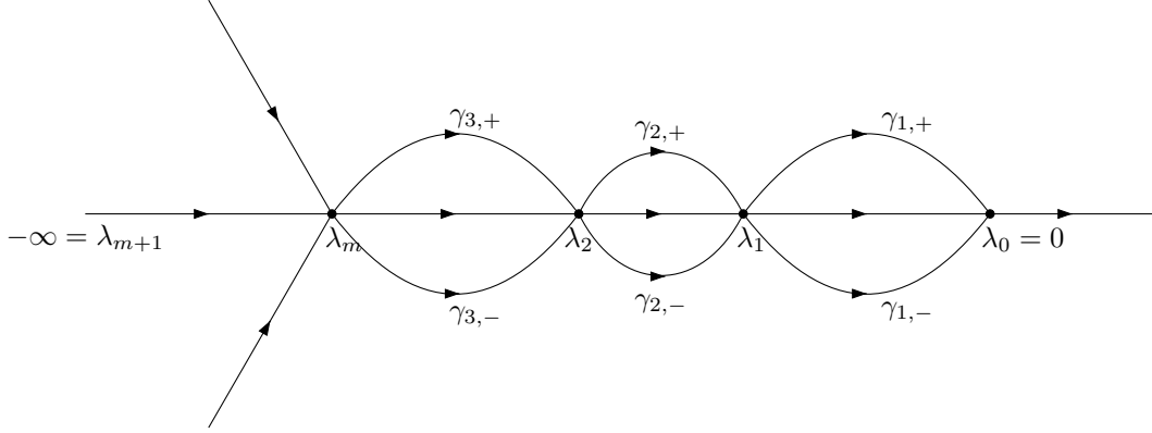
Figure 3: Jump contours \Gamma_S for S with m = 3 and s_1 > 0 .
