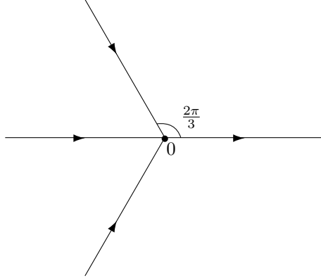
Figure 4: The jump contour \Sigma_A for \Phi_{\text{Ai}} .
