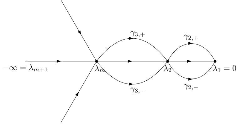
Figure 2: Jump contours \Gamma_S for S with m = 3 and s_1 = 0 .
